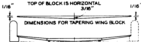
METHOD OF BLOCKING UP WING FOR DIHEDRAL
