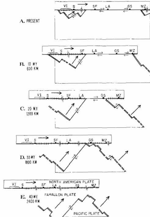
Figure 5. Schematic model of plate interactions assuming that the North American and Pacific plates moved with a constant relative motion of 6 cm/yr parallel to the San Andreas fault. The coast is approximated as parallel to the San Andreas. Farallon-Pacific plate motions are approximated from anomalies in Figure 1. Initials represent cities listed in Figure 6 and Vancouver Island. Boundaries and arrows are as in Figure 2, the Pacific plate being held fixed. Captions show the time represented by each sketch in millions of years before present and the distance that the North American plate must subsequently be displaced to reach its present position with respect to the Pacific plate.
