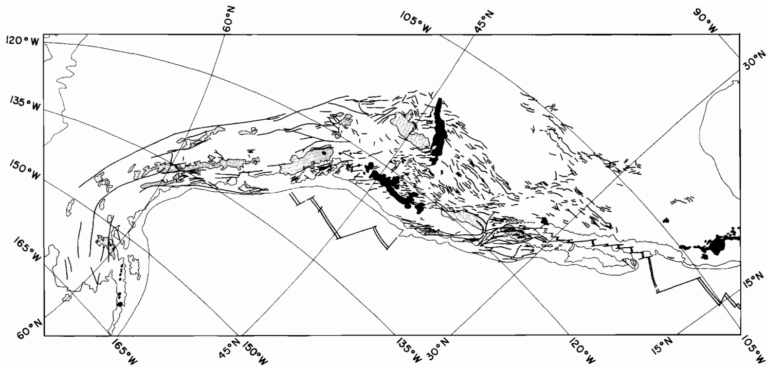
Figure 14. Some major tectonic features of western North America (after King, 1969). Quaternary volcanic rocks are black; granitic plutonic rocks are gray; most thrust faults have been omitted. Map projection is that used in Figure 4, so that deformation related to the motion between the American and Pacific plates can be imagined by keeping the ocean floor rigid and moving the rigid part of North America horizontally to the right. Horizontal faults experience pure strike slip while oblique faults have components of rifting or compression. A large-scale version of this projection is available from the author.
