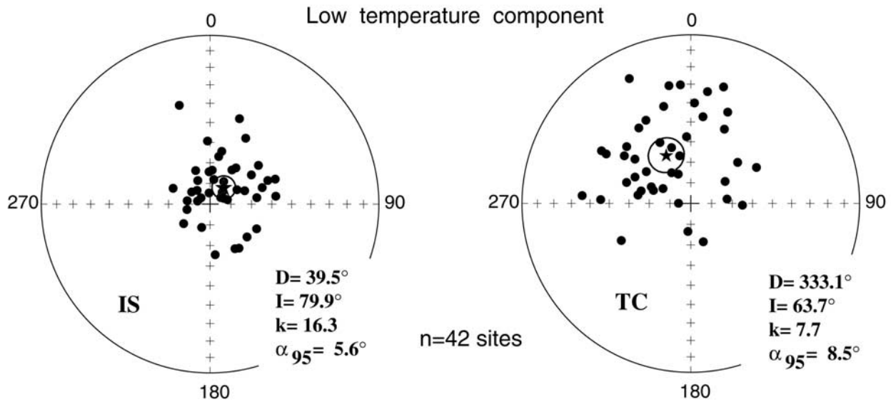
Figure 11. Equal-area projection of the low-temperature component site-mean directions (left) before and (right) after tilt correction.
