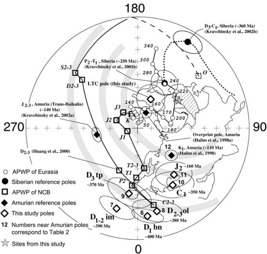
Figure 12. Equal-area projection of the northern hemisphere with the Devonian (Bolshoy Neaver ( D_1bn ), Imachi ( D_{1-2im} ), Oldoy ( D_{2-3ol} ), and Teplovka ( D_{3tp} ) formations), Early Carboniferous (Tipara formation ( C_1 )), and Middle Jurassic (Ayak formation ( J_2 )) from the present study (large dots with dp/dm ellipses of confidence) and from the literature [Halim et al., 1998a; Kravchinsky et al., 2002a, 2002b]. Small open dots, Eurasian APWP [Besse and Courtillot, 1991; Van der Voo, 1993] with ages indicated in Ma. Open diamonds, North China Block (NCB) APWP [Enkin et al., 1992; Gilder and Courtillot, 1997; Zhao et al., 1996] Grey curves are the small circles passing through this study poles and centered on site location (gray stars).
