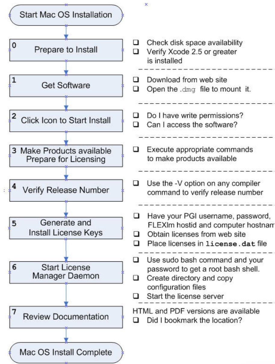
Figure 6.1. PGI Installation on Mac OS X Overview
