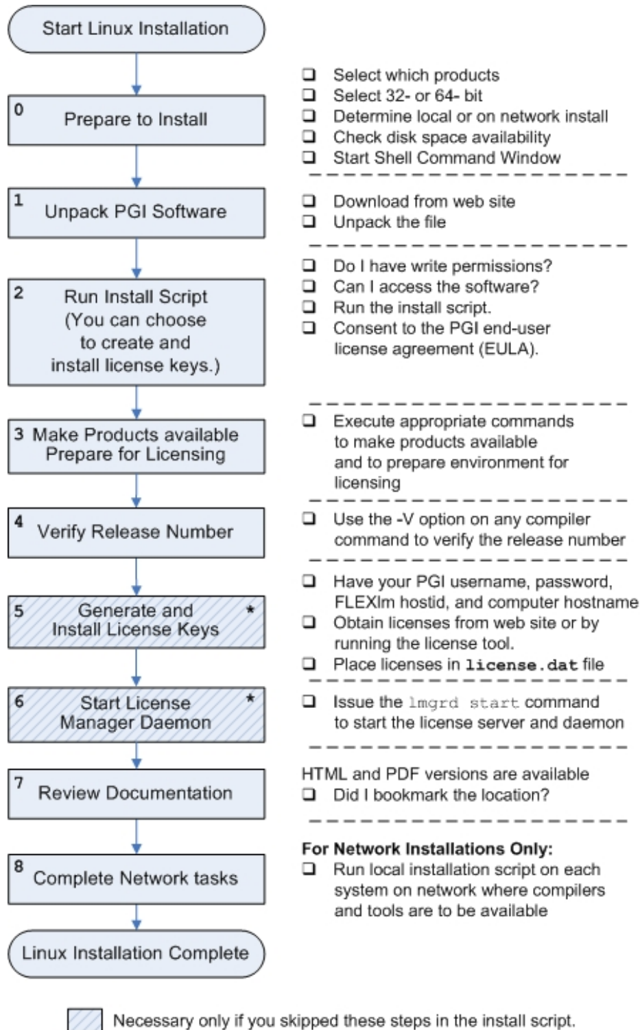
Figure 4.1. Linux Installation Overview
