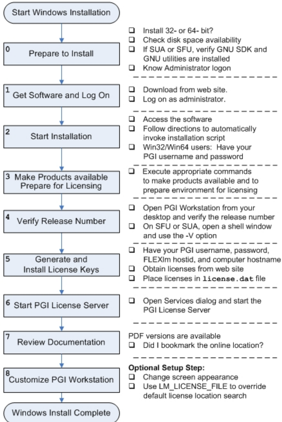
Figure 5.1. PGI Installation on Windows Overview
