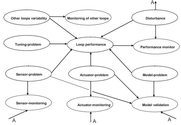
Fig. 3. A control loop monitoring and diagnosis architecture
