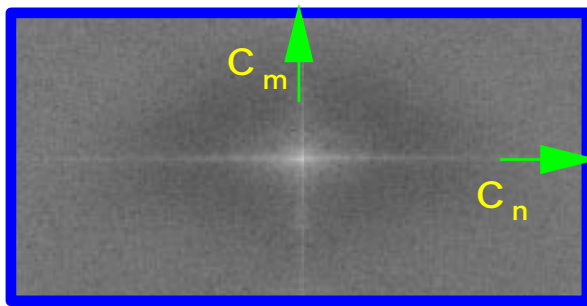
(Log of |c_{nm}|^2 )
