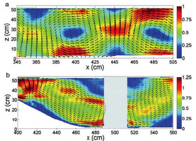
Figure 17. a) Left-to-right propagating vertical mode-1 internal waves generated using horizontally oscillating flat plates, as in Gostiaux et al. [2007]. b) Internal wave beam downstream of hill placed in front of the oncoming mode-1 waves. Adapted from Figures 2a and 3a of Peacock et al. [2009].
