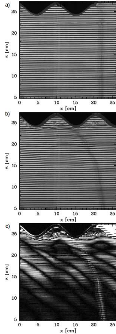
Figure 3. a) Side-view looking through tank filled with salt-stratified fluid with model inverted sinusoidal hills at the surface and an image of horizontal black and white lines placed behind the tank. b) Side-view after hills have been towed slowly a distance of one hill width. c) Qualitative synthetic schlieren image produced by taking the absolute value of the difference of the digitized images shown in a) and b). Also evident in a) and b) is a dark vertical streak above x \simeq 20 cm. This is a vertical dye-line suspended in the fluid itself. Its displacement can be used to determine mean horizontal flow, which is retrograde to the towing direction of the hill.
