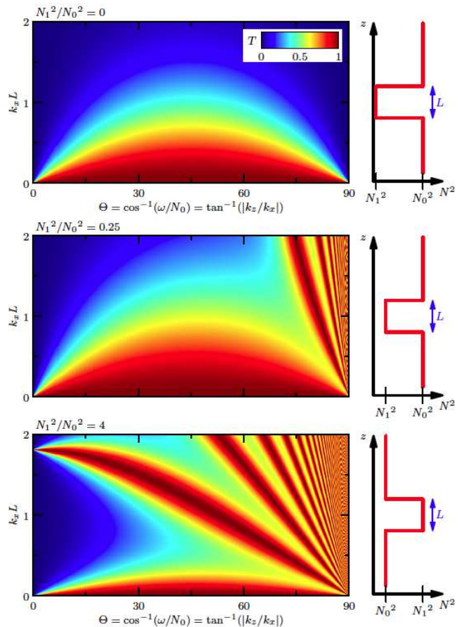
Figure 8. Predicted transmission coefficient for monochromatic internal waves of frequency \omega and horizontal wavenumber k_x , incident upon a region of depth L where the ambient buoyancy frequency is N_1 instead of N_0 . Adapted from Figure 1 of Sutherland and Yewchuk [2004].
