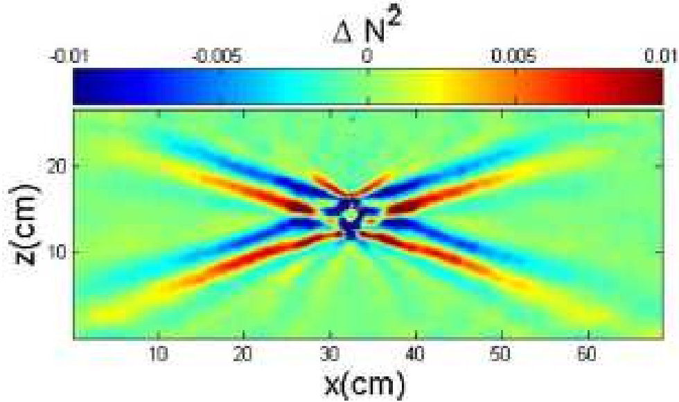
Figure 5. Change in the background squared buoyancy frequency ( \Delta N^2 ) due to internal waves generated by an oscillating cylinder, as measured by quantitative synthetic schlieren. The left image shows a snapshot of the \Delta N^2 field; the right image shows the amplitude envelope of the wave beams. Reproduced from Figure 2 of Mercier et al. [2008].
