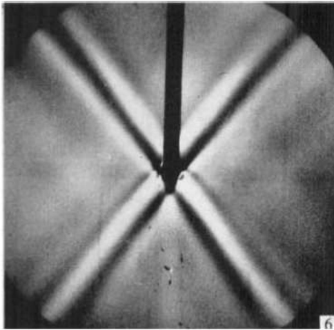
Figure 2. Pattern of internal waves generated by an oscillating cylinder as visualized by conventional schlieren methods. Reproduced from Plate 1(6) of Mowbray and Rarity [1967].
