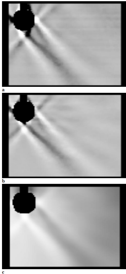
Figure 7. Quantitative synthetic schlieren applied to the circumstance shown in Figure 4, in which a) the horizontal displacement of dots behind the tank is used to compute the (assumed spanwise-uniform) horizontal perturbation density gradient of fluid in the tank, as indicated by intensity of the gray scale. In b) vertical dot displacements are used to compute the vertical density gradient. In c) the two components of the density gradient are integrated to find the perturbation density field. Reproduced from Figure 13 of Dalziel et al. [2000].
