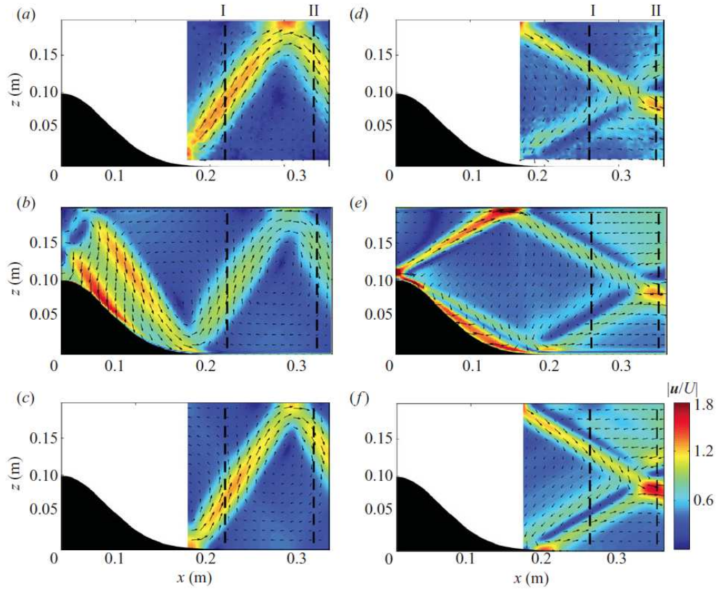
Figure 18. Experimental measurements (top), numerical results (middle) and theoretical predictions (bottom) of internal waves generated by oscillatory flow over a Gaussian hill in cases where the frequency of oscillation is subcritical (left) and supercritical (right). Reproduced from Figure 2 of Echeverri et al. [2009].
