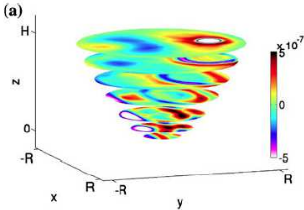
Figure 13. Tomographic reconstruction of internal wave field inside an oscillating parabolic domain computed from many views of image displacements like those in Figure 12. Reproduced from Figure 4a of Hazewinkel et al. [2011].
