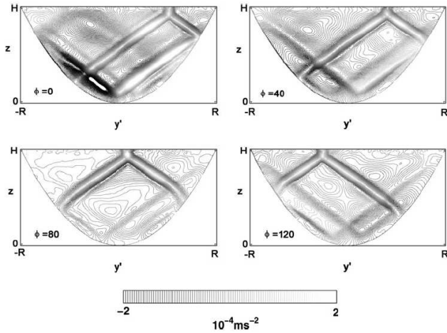
Figure 12. Image displacements recorded by different perspectives looking horizontally through an oscillating paraboloid filled with uniformly stratified fluid. Reproduced from Figure 2 of Hazewinkel et al. [2011].
