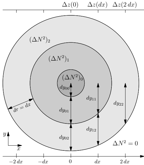
Figure 10. Discretization used to represent apparent displacements in an image behind a tank to axisymmetric disturbances within the tank. The disturbances are represented in terms of changes to the squared buoyancy frequency \Delta N^2 , which is assumed constant on annuli of width dr = dx , in which dx is the horizontal (e.g. pixel) resolution of the observed vertical displacements \Delta z of the object image.
