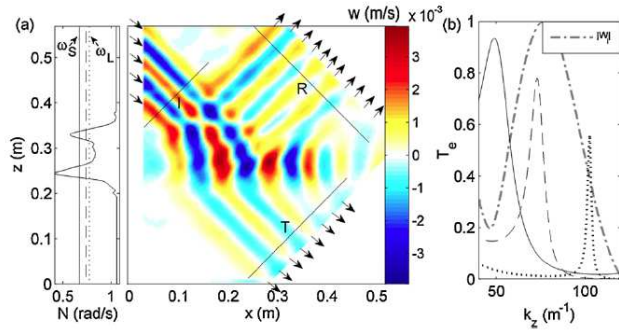
Figure 9. Schlieren image (colour) showing the vertical velocity field associated with incident internal waves in non-uniformly stratified media, partially transmitting (indicated by ‘T’) and reflecting (indicated by ‘R’) with partial trapping in a region of locally enhanced stratification. The profile of the background stratification is shown to the left and transmission spectra are shown to the right. Adapted from Figure 3 of Mathur and Peacock [2010].
