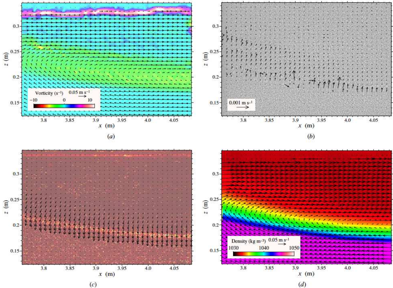
Figure 15. a) Vorticity, b) uncorrected displacements, c) corrected displacements and d) density field resulting from the passage of an internal solitary wave of depression in an approximately two-layer fluid. Reproduced from Figure 12 of Dalziel et al. [2007].
