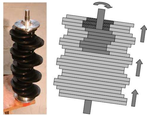
Figure 16. Camshaft and schematic cross-section showing how the rotation of the shaft results in the back and forth oscillation of flat plates. Reproduced from Figure 2 of Gostiaux et al. [2007].
