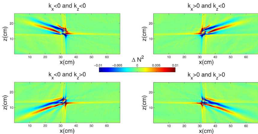
Figure 6. The four arms of the cross shown in Figure 5 determined by Fourier implementation of the Hilbert Transform. Reproduced from Figure 3 of Mercier et al. [2008].
