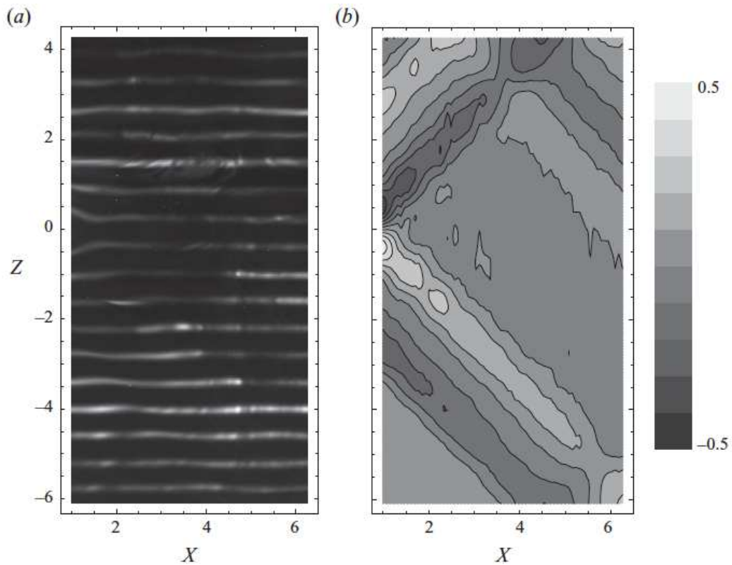
Figure 19. a) Dye lines displaced to the right of a sphere oscillating horizontally about the origin in uniformly stratified fluid and b) computed displacement of the lines relative to the oscillating amplitude A . Reproduced from Figure 20 of Voisin et al. [2011].
