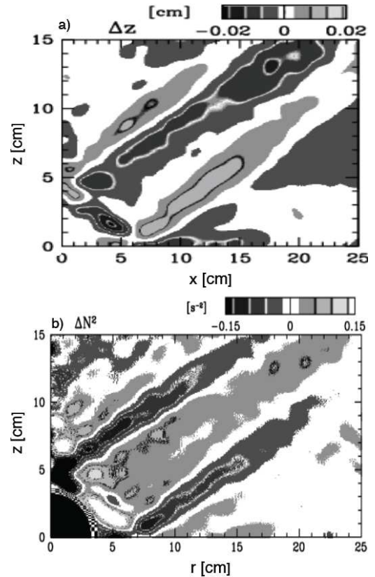
Figure 11. a) Apparent vertical displacement, \Delta z(x, z) of horizontal lines in an image behind a tank in which a sphere (situated to the bottom left) oscillates in uniformly stratified fluid. b) Corresponding change in squared buoyancy frequency, \Delta N^2(r, z) , due to internal waves computed through axisymmetric synthetic schlieren. Adapted from Figures 2b and 4a of Onu et al. [2003].
