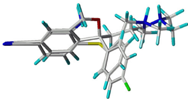
Figure 2: Alignment of DASB and (S)-citalopram generated by using GASP.
