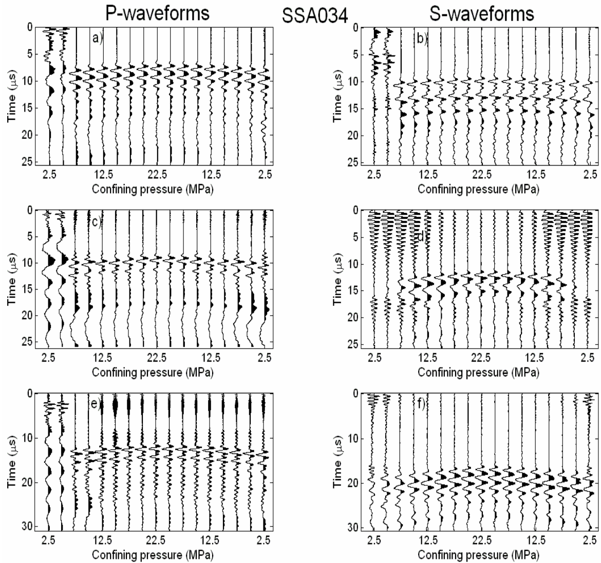
Figure A.17 – Complete suite of waveforms obtained for the 2 nd White Specks sandstone.
