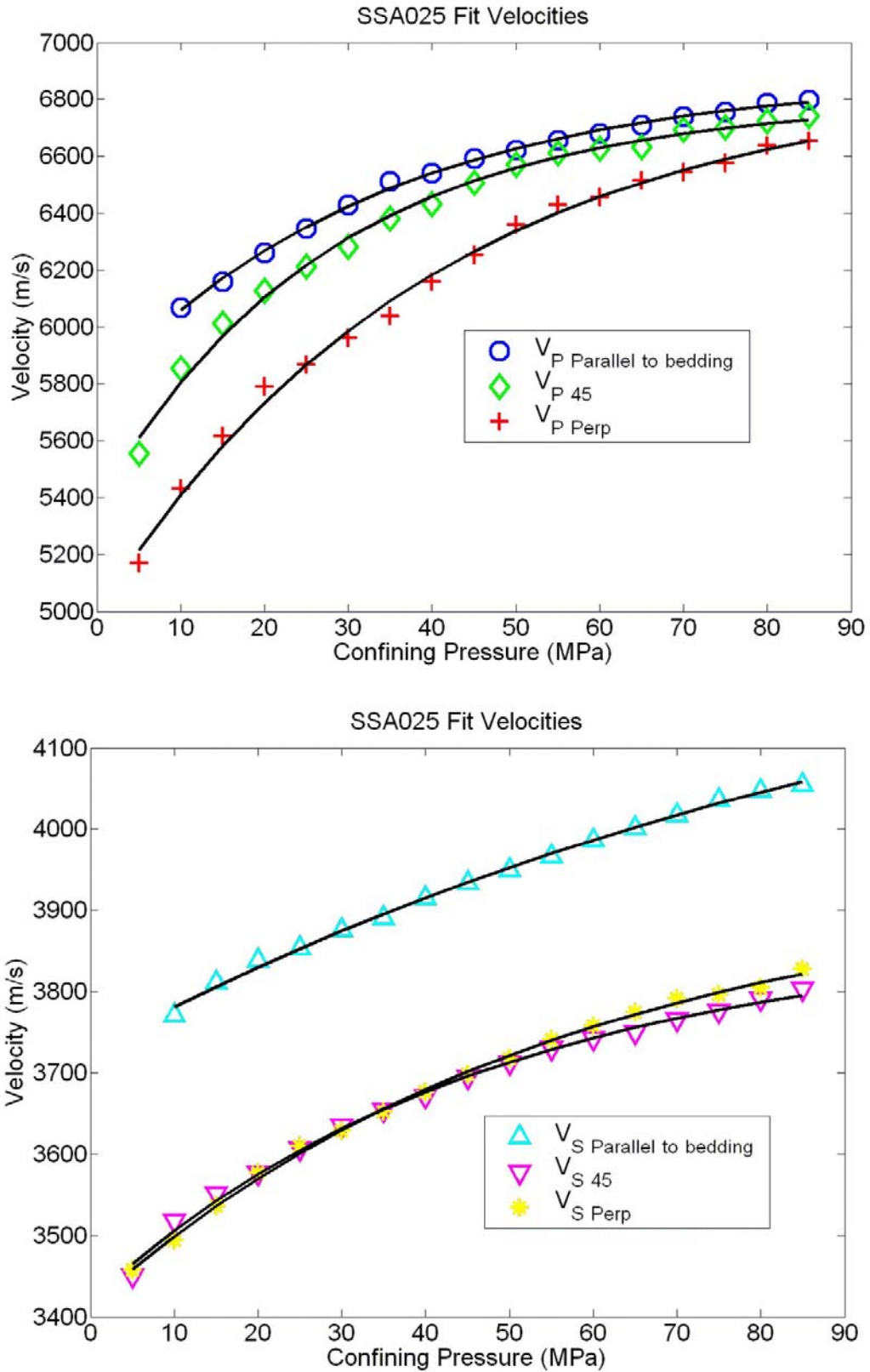
Figure 5.6 - Fits of the velocities of the Wabamun carbonate using Equation 5.1.
