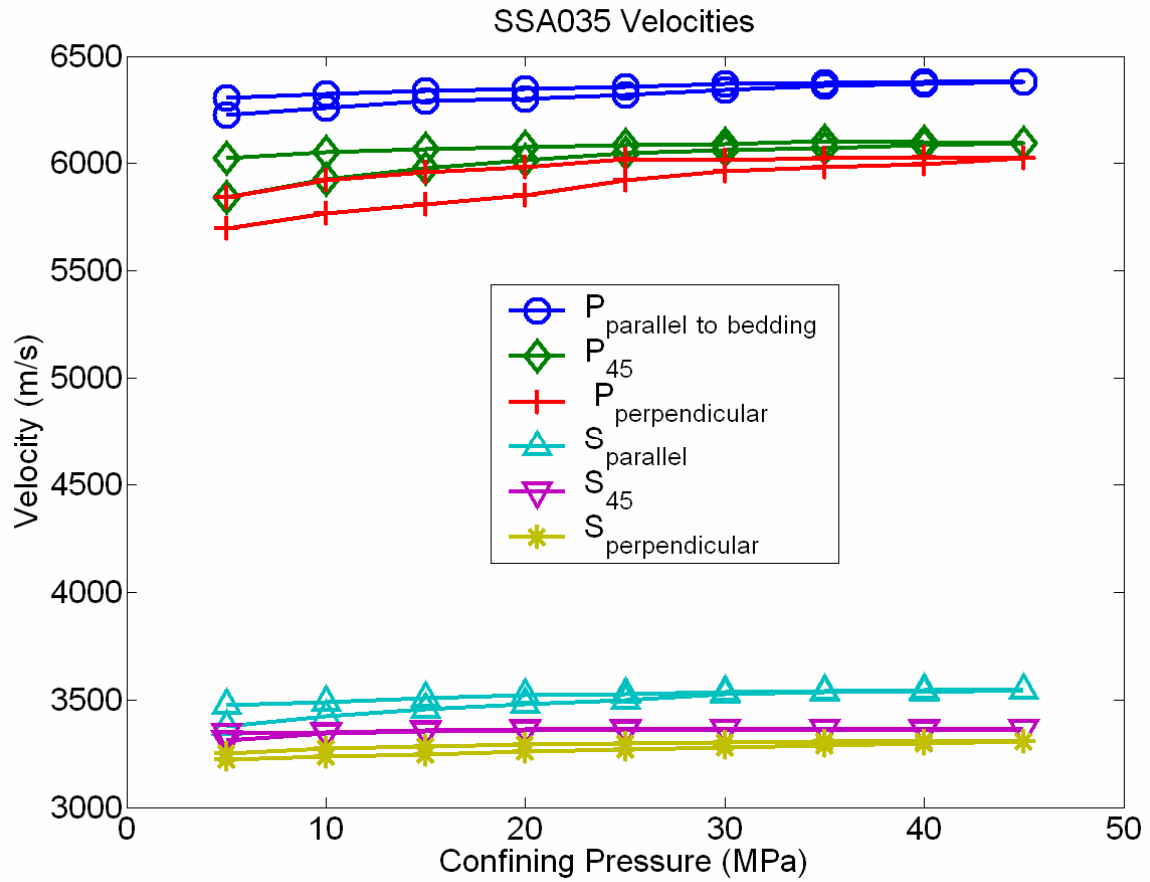
Figure A.22 - Velocities for the Big Valley anhydrite.
