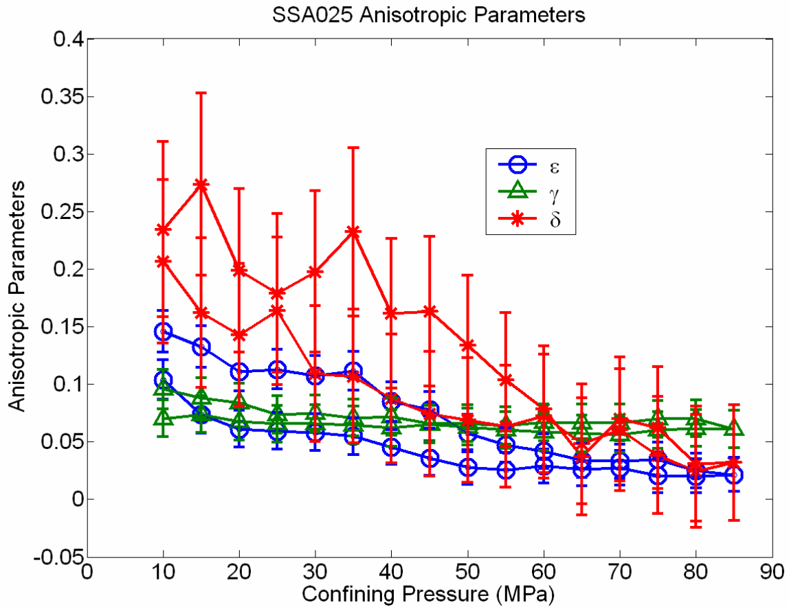
Figure A.16 - Anisotropic parameters for the Wabamun carbonate.
