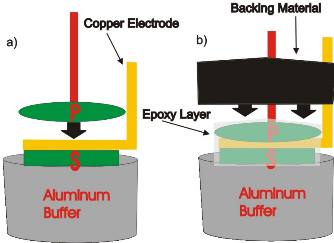
Figure 3.1 - The steps necessary to build the transducers. a) First the P-wave transducer is stacked onto the S-wave transducer with a copper electrode between them. b) The ceramics are then coated with a thin layer of epoxy. The entire back of the aluminum buffer is then coated with a damping material of urethane rubber and iron filings.
