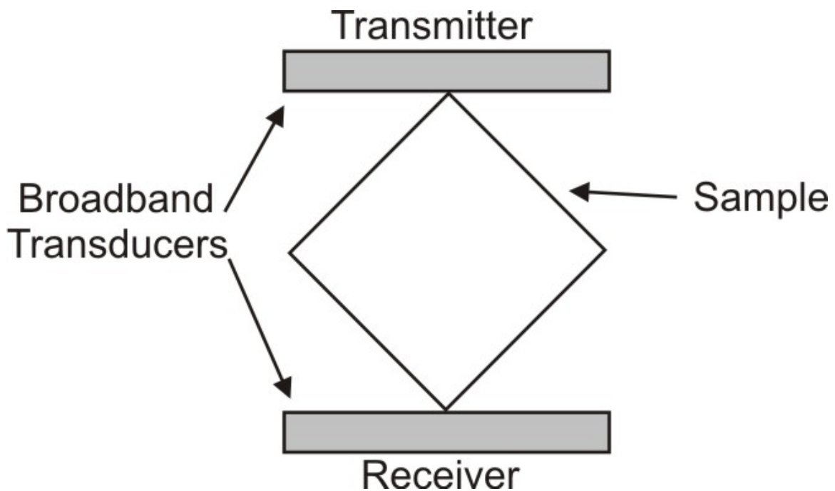
Figure 2.8 - A RUS experimental setup at ultrasonic frequencies. The sample, a few millimeters in size, is held lightly between two broadband transducers. Resonance modes are found in order to determine the elastic constants.
