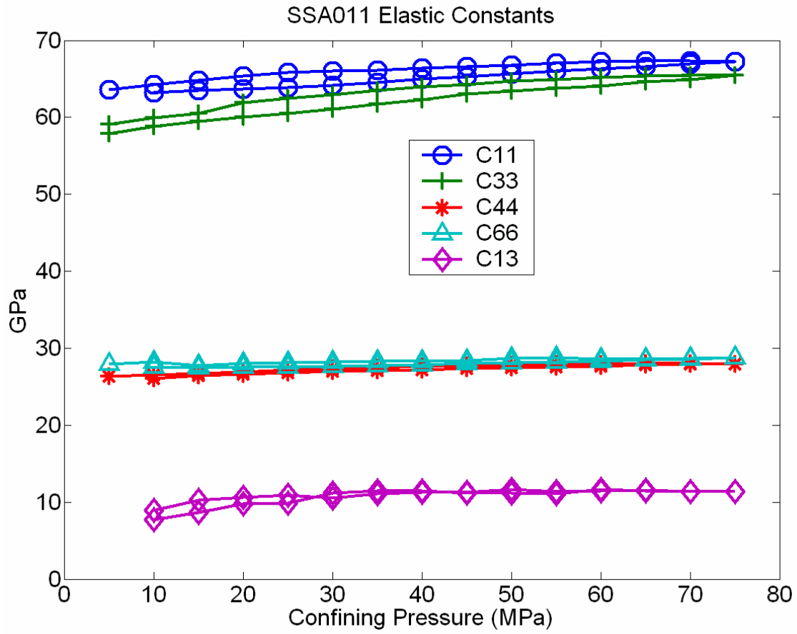
Figure A.7 - Elastic constants of the Mannville shale 2.
