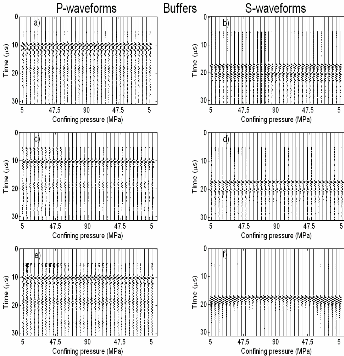
Figure 3.6 – Waveform suites of the buffers. a) and b) show the P- and S-waves, respectively, in the 12 buffer set. c) and d) show the waveforms in the 34 set, and e) and f) show the waveforms in the 56 set. There is almost no pressure dependence.
