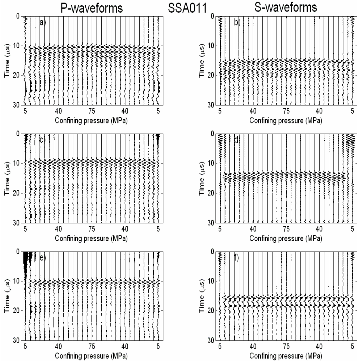
Figure A.5 – Complete suite of waveforms obtained for the Mannville shale 2. a) and b) show the P- and S-waves, respectively, traveling perpendicular to bedding. c) and d) show the waveforms traveling 45° to bedding, and e) and f) show the waveforms parallel to bedding.
