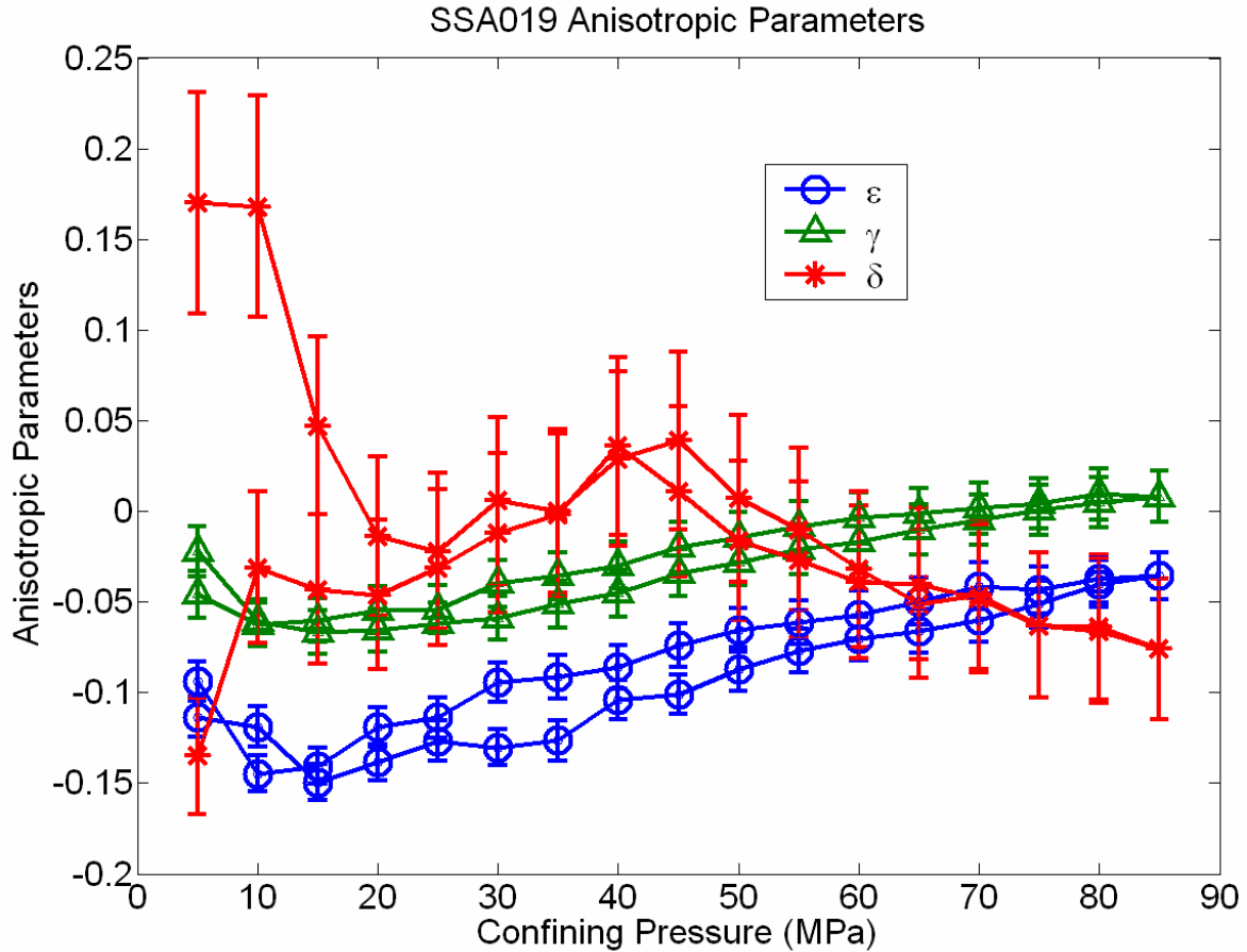
Figure 5.8 - Anisotropic parameters of the Mount Head carbonate.
