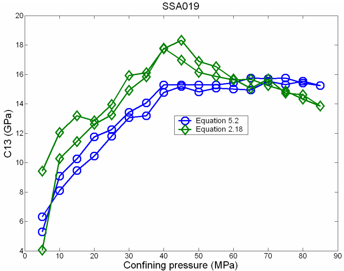
Figure 5.12 - C_{13} for the Mount Head carbonate calculated using Equation 2.18 and 5.2.
