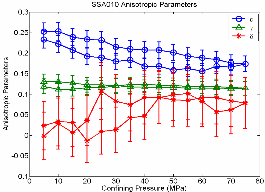
Figure 5.9 - Anisotropic parameters for the Mannville shale 1.
