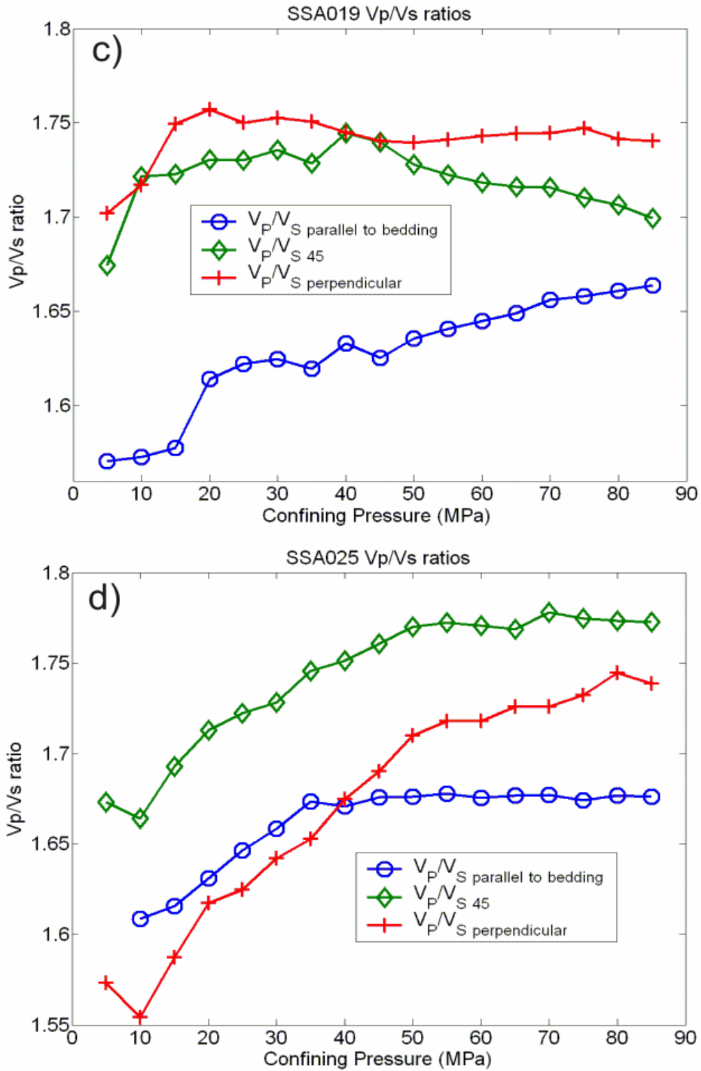
Figure 5.13 (continued) - V_p/V_s ratios for c) the Mount Head carbonate (SSA019) and d) the Wabamun carbonate (SSA025).
