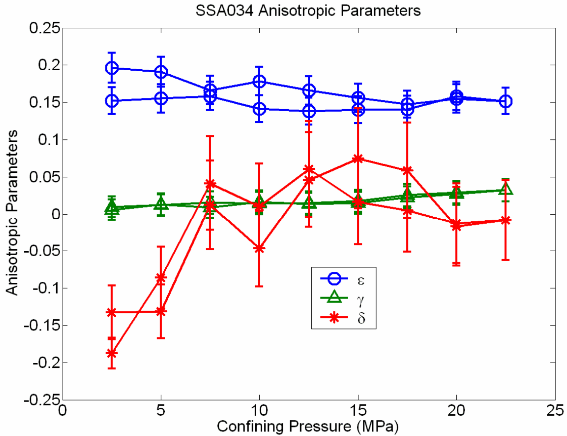
Figure A.20 – Anisotropic parameters for the 2 nd White Specks sandstone.
