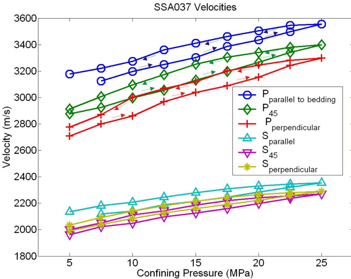
Figure 5.2 - Velocities of the Bow Island sandstone. Arrows on the P-waves indicate the progression of measurements. Arrows on the S-waves are omitted for clarity. Velocities are higher while decreasing pressure.
