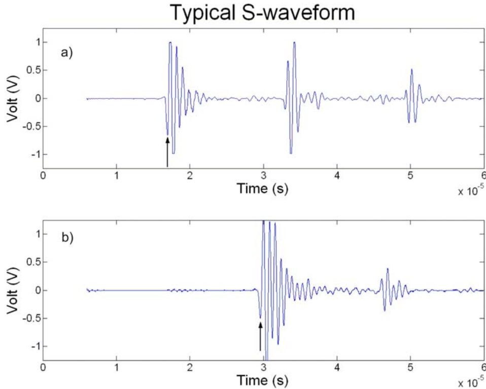
Figure 3.5 - The signal through a) the buffers and b) the buffers and sample. The travel time is picked at the first extremum, marked by arrows. To obtain the travel time through the sample, the time in a) is subtracted from the time in b).
