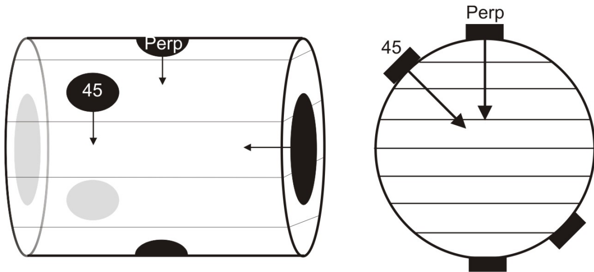
Figure 2.6 - The single-core method developed by Wang (2002a) for use on TI materials. A core is cut parallel to bedding and transducers are affixed to either end to measure the velocity parallel to bedding. Transducers used to measure velocities perpendicular and 45° to bedding are fit into a rubber jacket that is placed around the sample.
