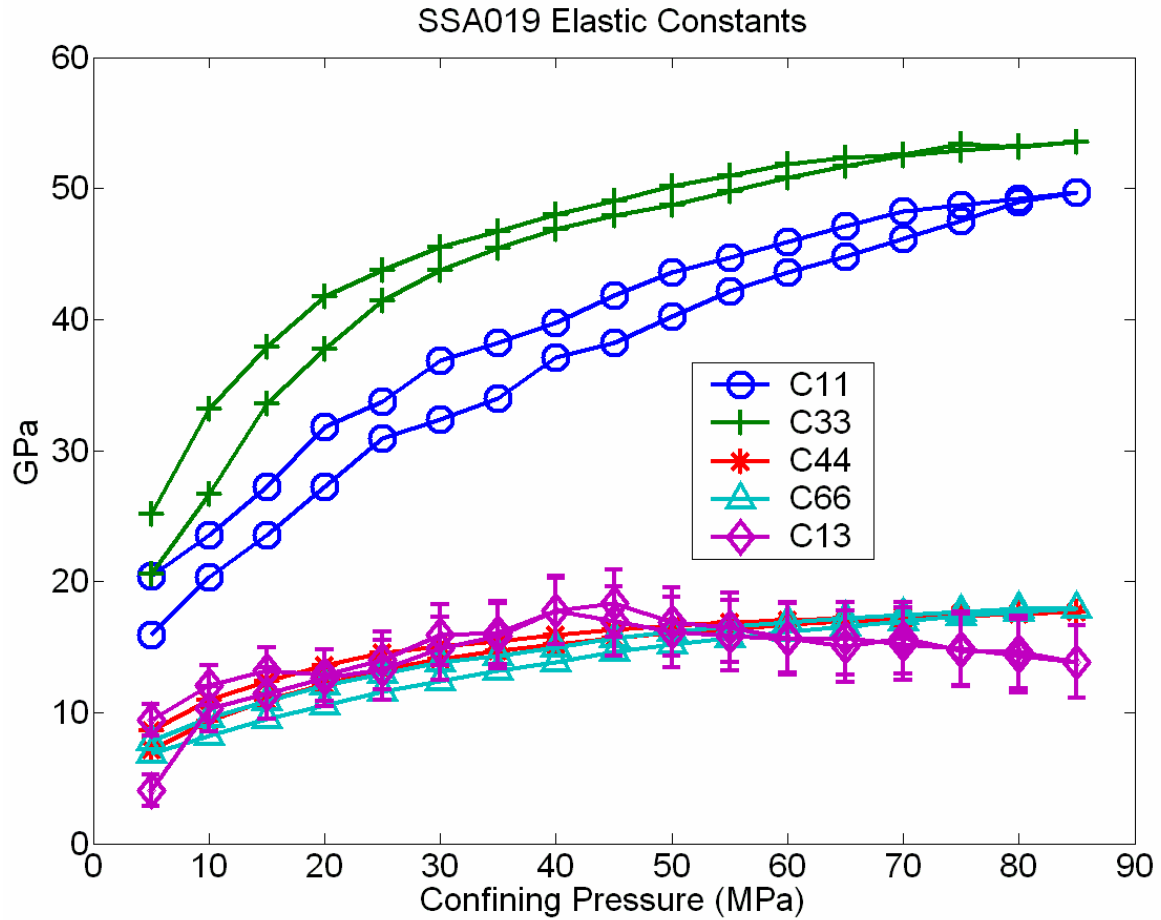
Figure 5.11 – Elastic constants for the Mount Head carbonate. Error bars are included for C_{13} .
