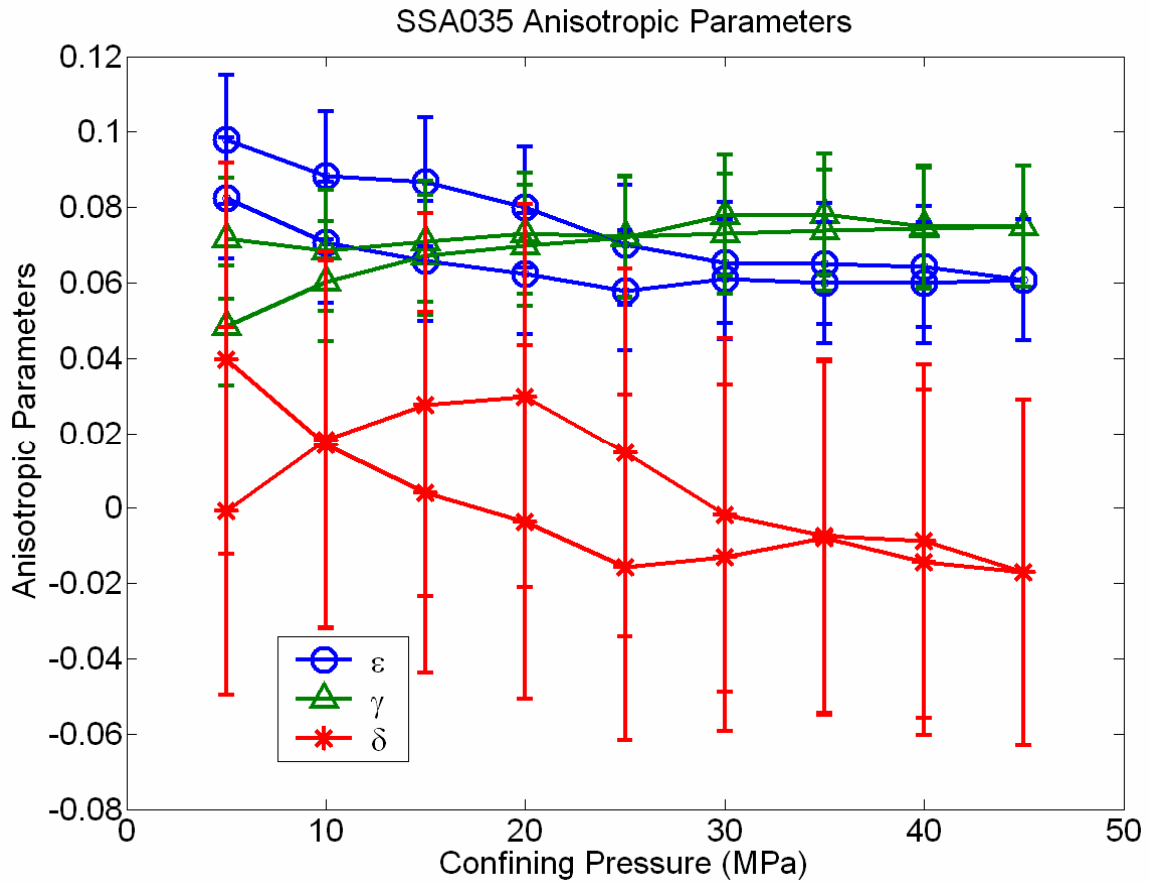
Figure A.24 - Anisotropic parameters for the Big Valley anhydrite.
