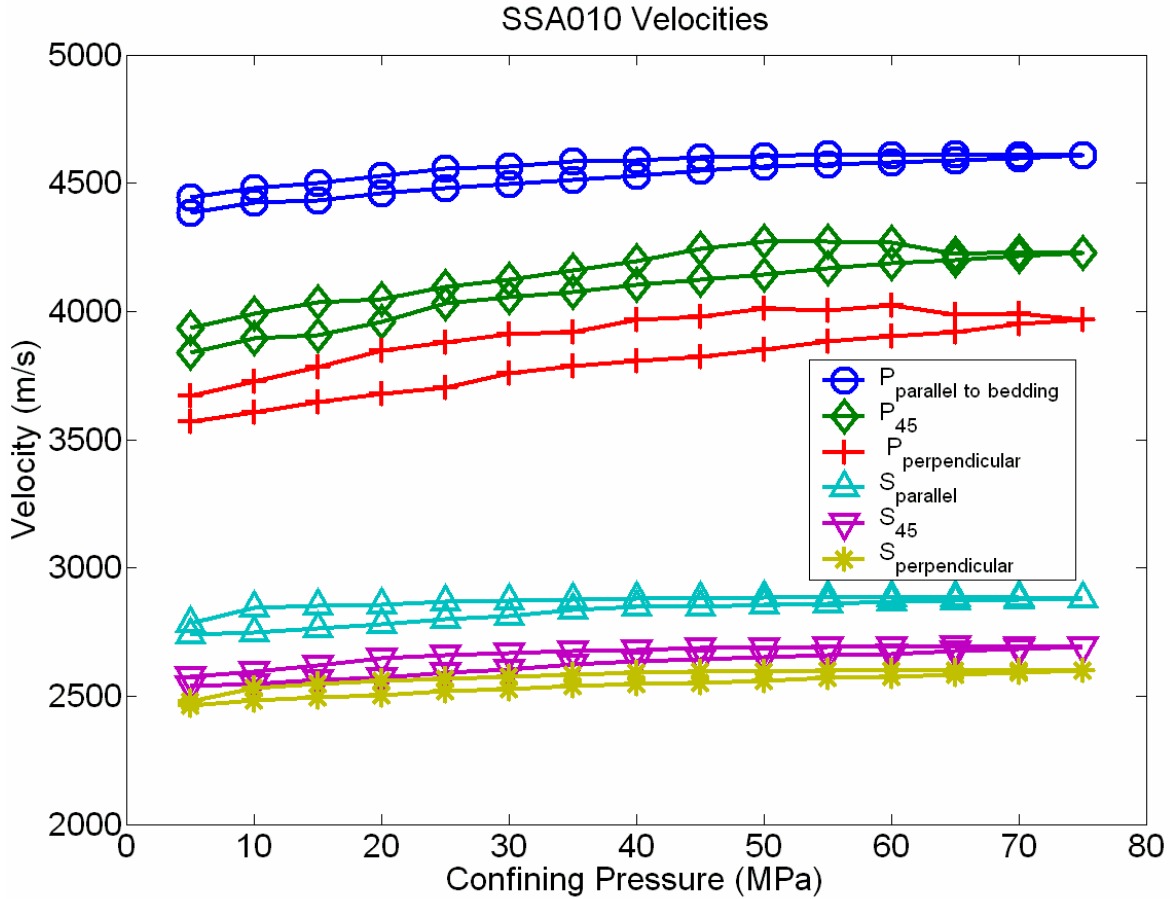
Figure 5.4 - Velocities of the Mannville shale 1. The velocities are relatively stable over the pressure range.
