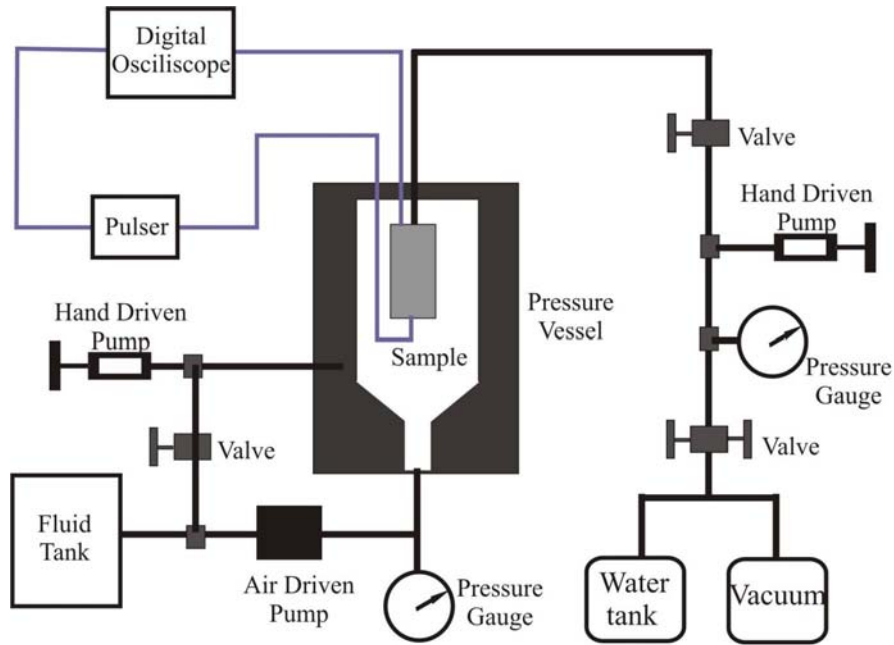
Figure 3.4 - A schematic of the experimental setup. The sample was placed in the pressure vessel and pulsed with the pulser. The oscilloscope read the signal. Pressure was provided from an air driven pump and fine tuned with a hand driven pump. The pore pressure equipment was not used in this set of experiments. Figure modified after He (2006).
