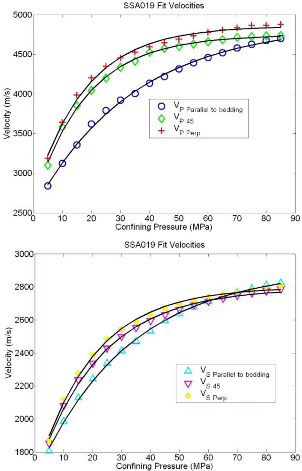
Figure 5.5 - Fits of the velocities of the Mount Head carbonate using Equation 5.1.
