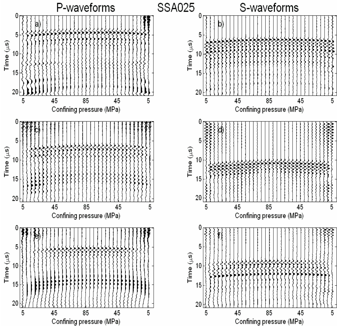
Figure A.13 – Complete suite of waveforms obtained for the Wabamun carbonate. a) and b) show the P- and S-waves, respectively, traveling perpendicular to bedding. c) and d) show the waveforms traveling 45^\circ to bedding, and e) and f) show the waveforms parallel to bedding.
