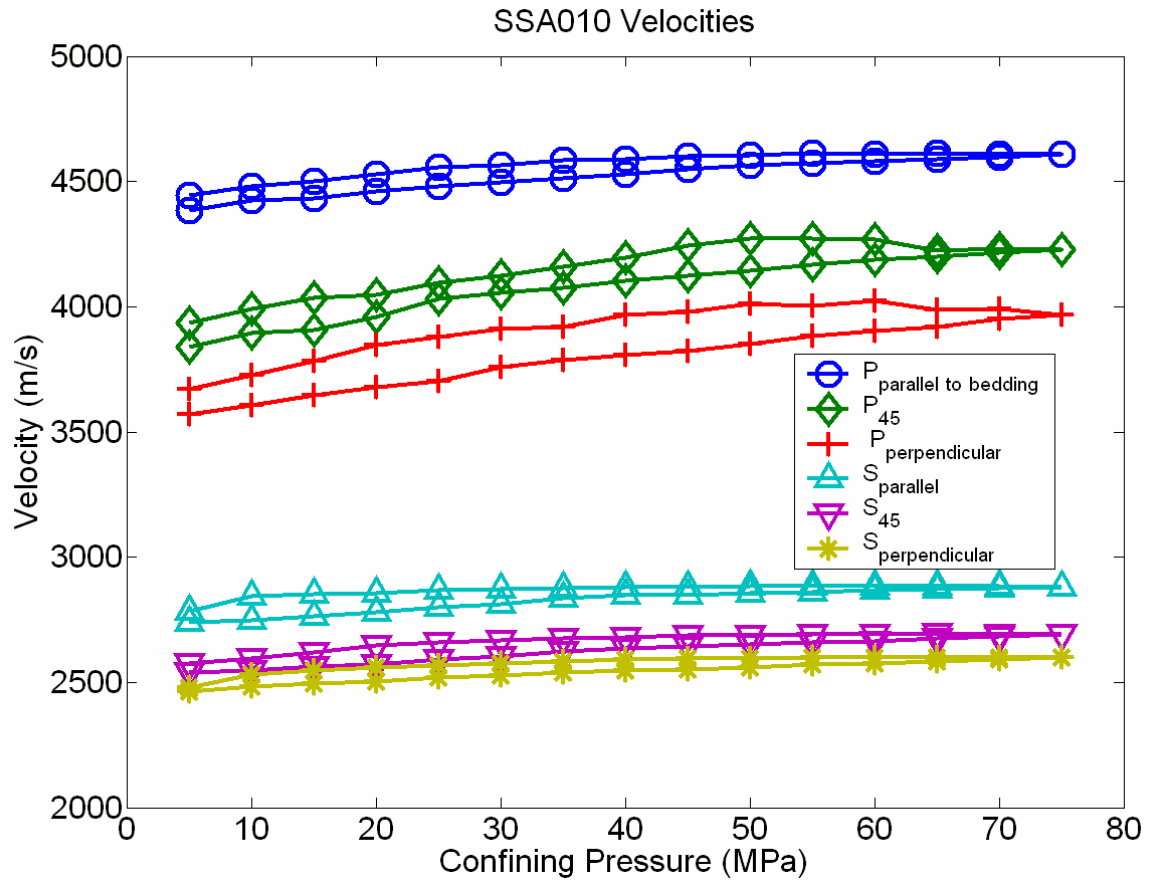
Figure A.2 - Velocities for the Mannville shale 1.
