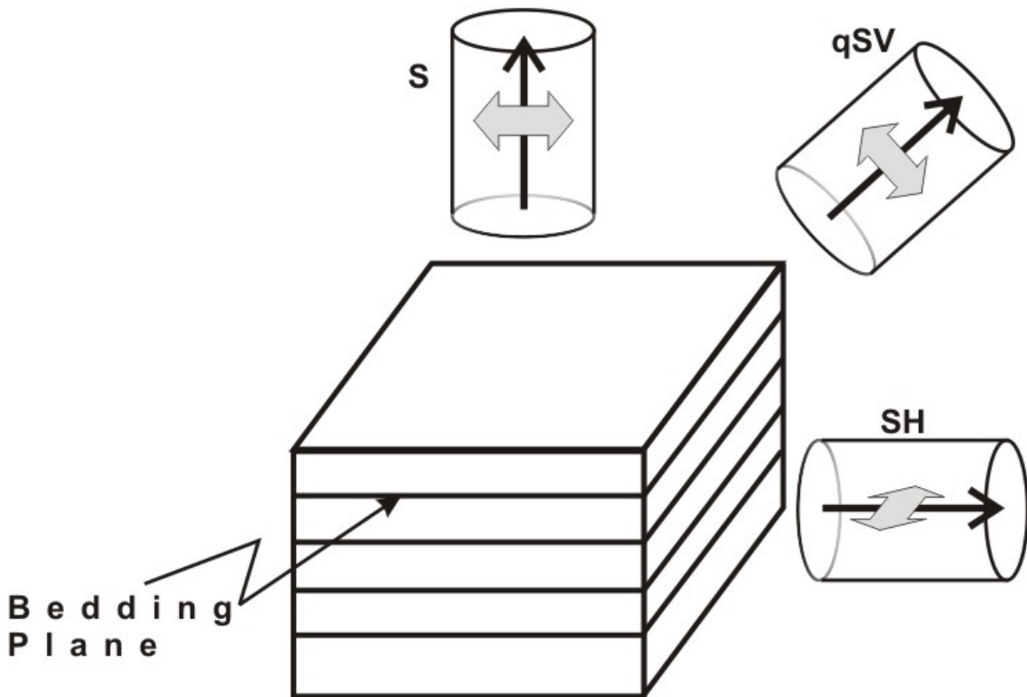
Figure 2.4 - The propagation direction and polarization of waves measured in the multi-core method in TI rocks. The SH-wave is found in the core cut parallel to bedding while the qSV-wave is found in the core cut 45° to bedding. The polarization of the S-wave traveling perpendicular to bedding is irrelevant because of symmetry. P-waves are found on all cores.
