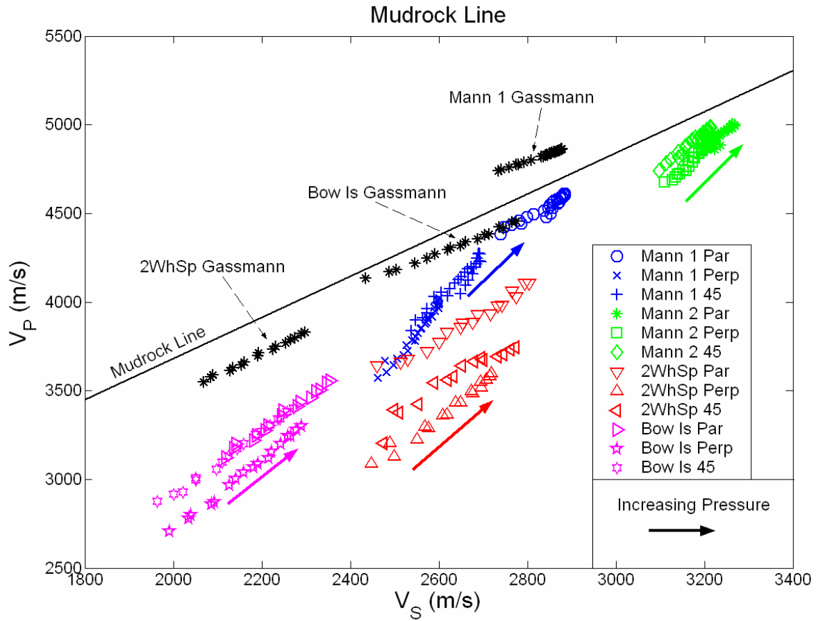
Figure 5.14 - V_P versus V_S for the shale and sandstone samples. The black line is the mudrock line defined by Castagna et al. (1985). The black asterisk symbols are the Gassmann substituted points using velocities parallel to bedding. No Gassmann substitution was performed on the Mannville shale 2 due to its very low porosity.
