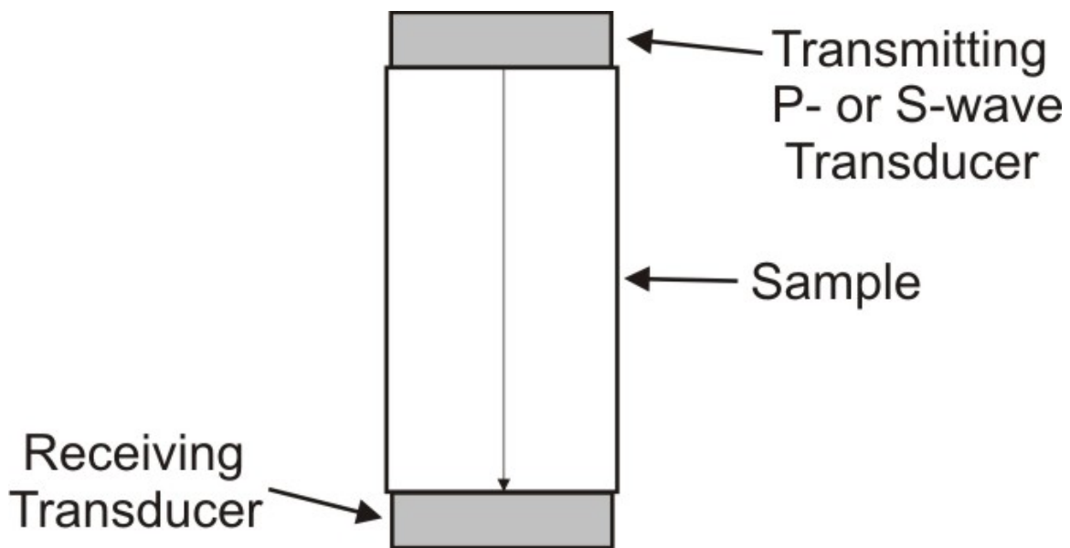
Figure 2.3 - The basic premise of a pulse-transmission experiment. A transmitting transducer sends a wave through the sample where it is recorded by a receiving transducer.
