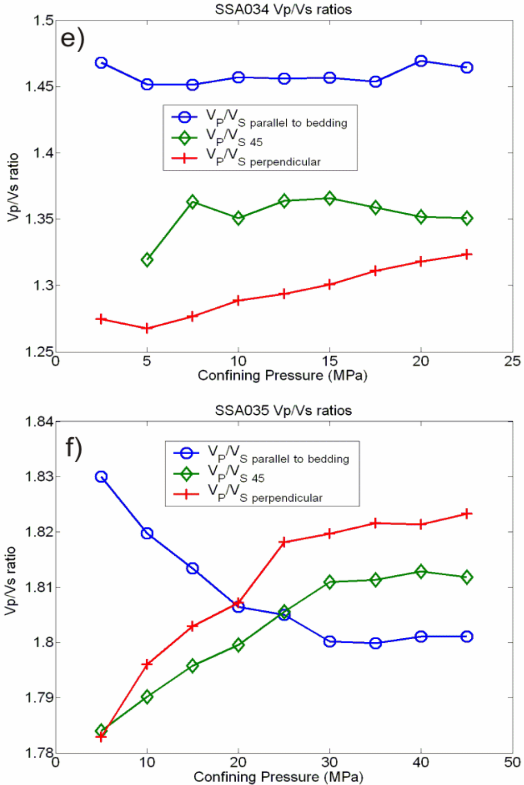
Figure 5.13 (continued) - V_p/V_s ratios for e) the 2 nd White Specks sandstone (SSA034) and f) the Big Valley anhydrite (SSA035).
