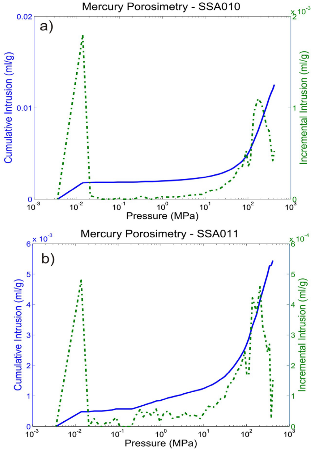
Figure 4.4 - Cumulative and incremental intrusion curves for the a) Mannville shale 1 (SSA010) and b) Mannville shale 2 (SSA011).
