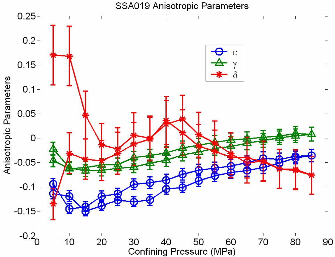
Figure A.12 - Anisotropic parameters of the Mount Head carbonate.
