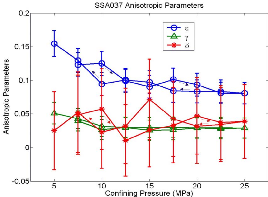
Figure 5.7 - Anisotropic parameters of the Bow Island sandstone. Measurements made while increasing pressure are the upper curves. Progression is marked by arrows.
