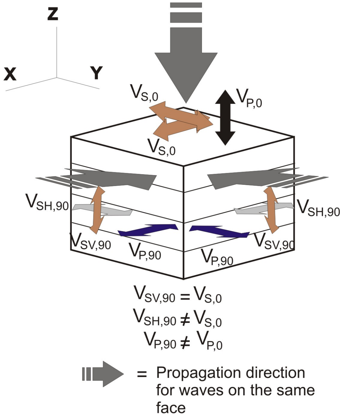
Figure 2.1 – The symmetry of a TI medium. Elastic properties are symmetric about the Z-axis. Waves are propagating into the face of the cube that they are located on. Waves of the same colour propagate with the same speed. The vertically polarized S-wave propagating 90° from the symmetry axis propagates at the same speed as the S-wave traveling parallel to the symmetry axis. See text for more details.
