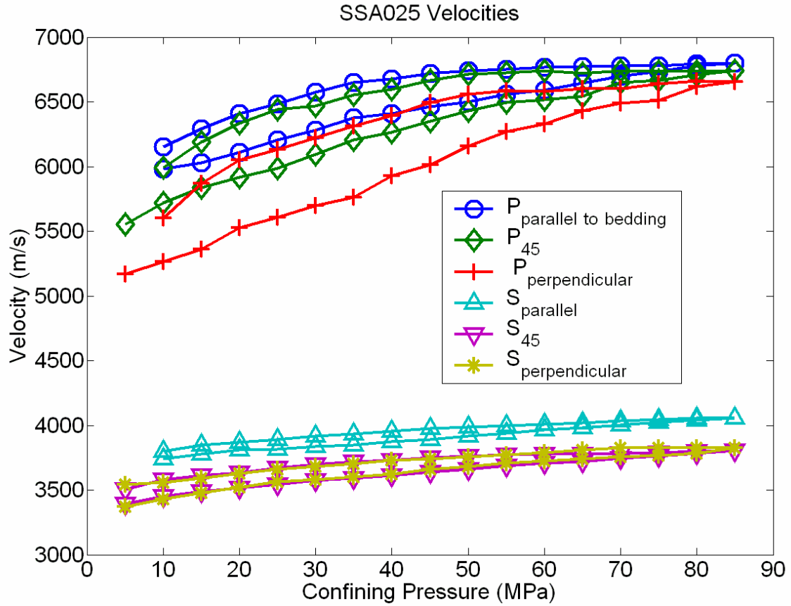
Figure A.14 - Velocities of the Wabamun carbonate.
