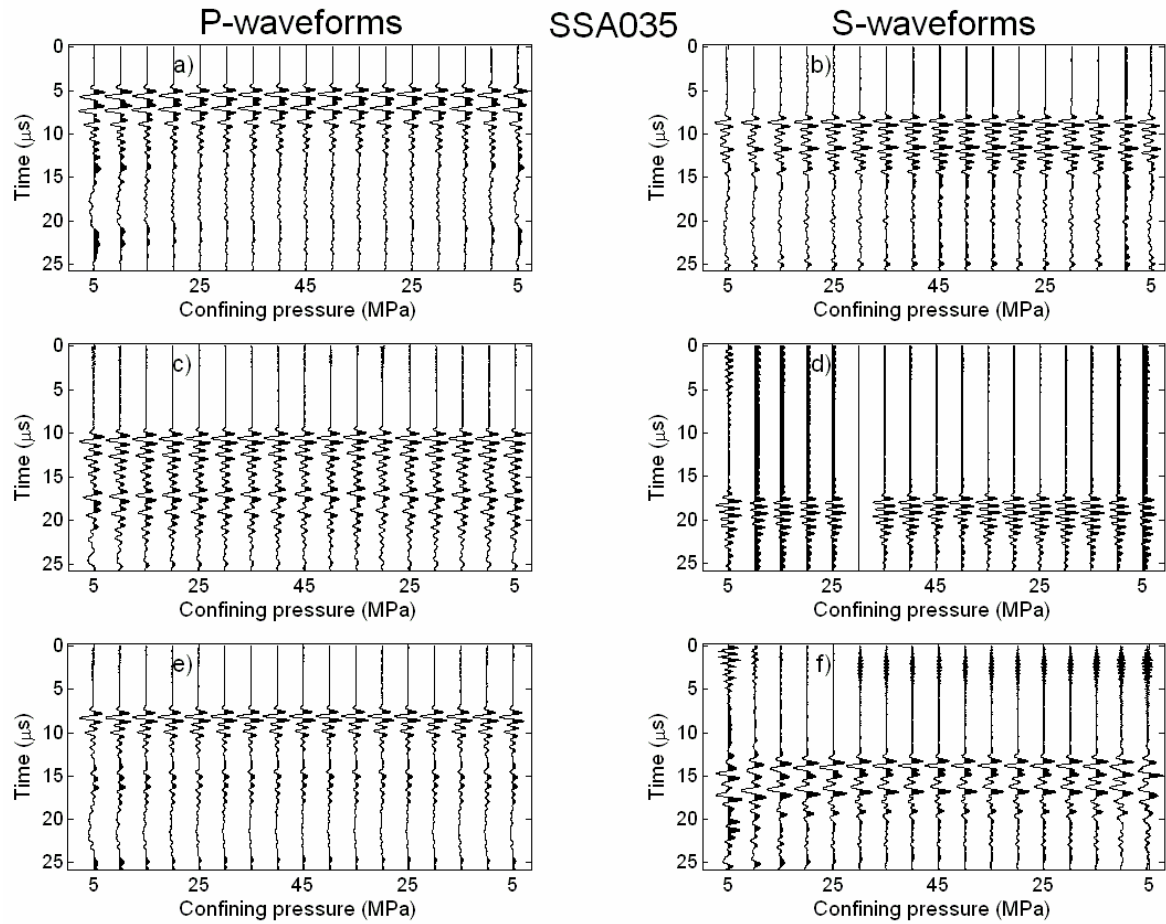
Figure A.21 – Complete suite of waveforms obtained for the Big Valley anhydrite. a) and b) show the P- and S-waves, respectively, traveling perpendicular to bedding. c) and d) show the waveforms traveling 45^\circ to bedding, and e) and f) show the waveforms parallel to bedding.
