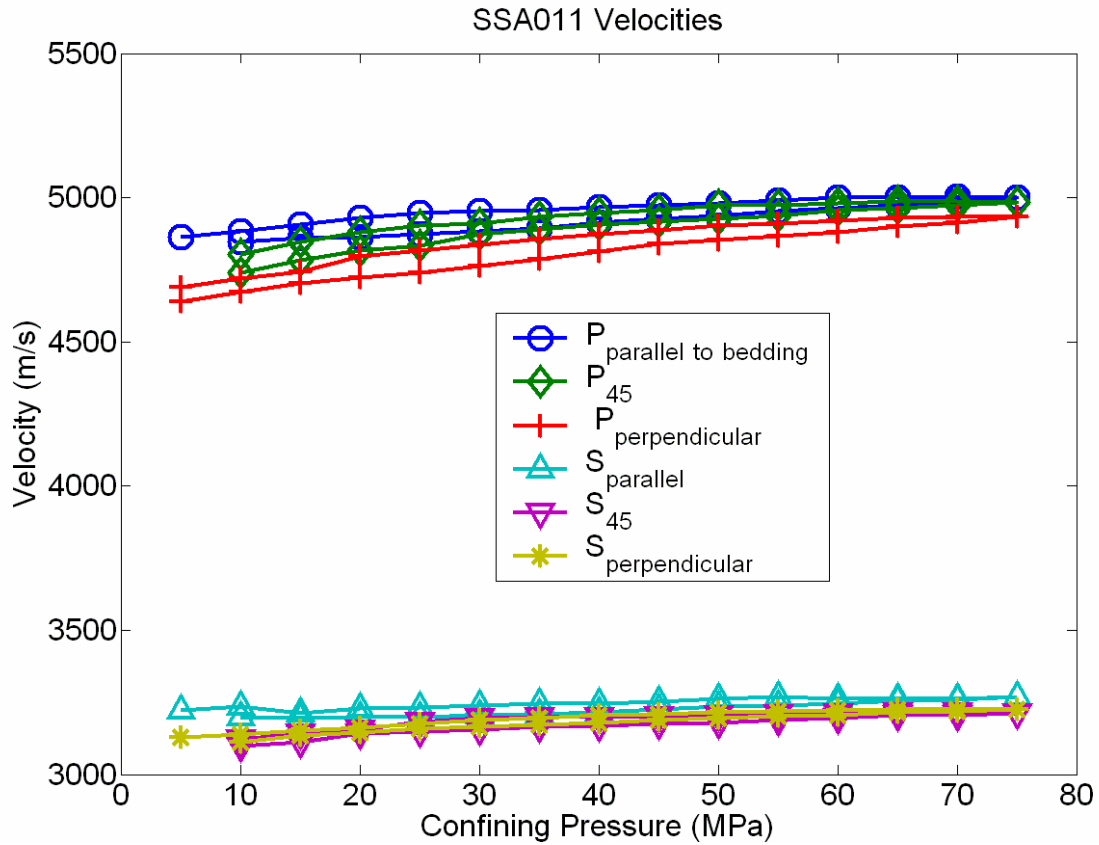
Figure A.6 - Velocities for the Mannville shale 2.
