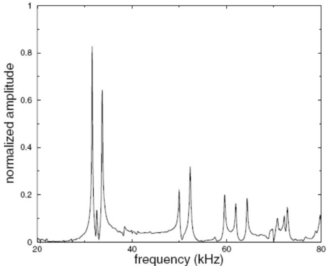
Figure 2.9 - Amplitude versus frequency spectrum of a cylindrical granite core (2.527 cm diameter and 7.15 cm long). Figure from Zadler et al. (2004) with permission to use granted by Blackwell Publishing.
