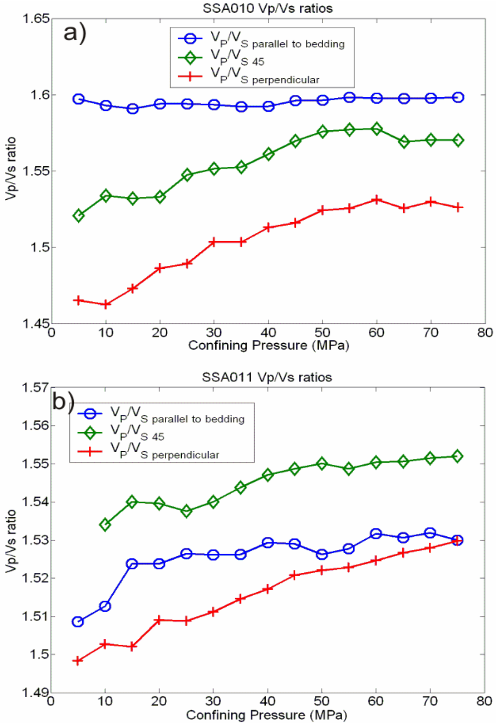
Figure 5.13 - V_p/V_s ratios for a) the Mannville shale 1 (SSA010) and b) the Mannville shale 2 (SSA011).
