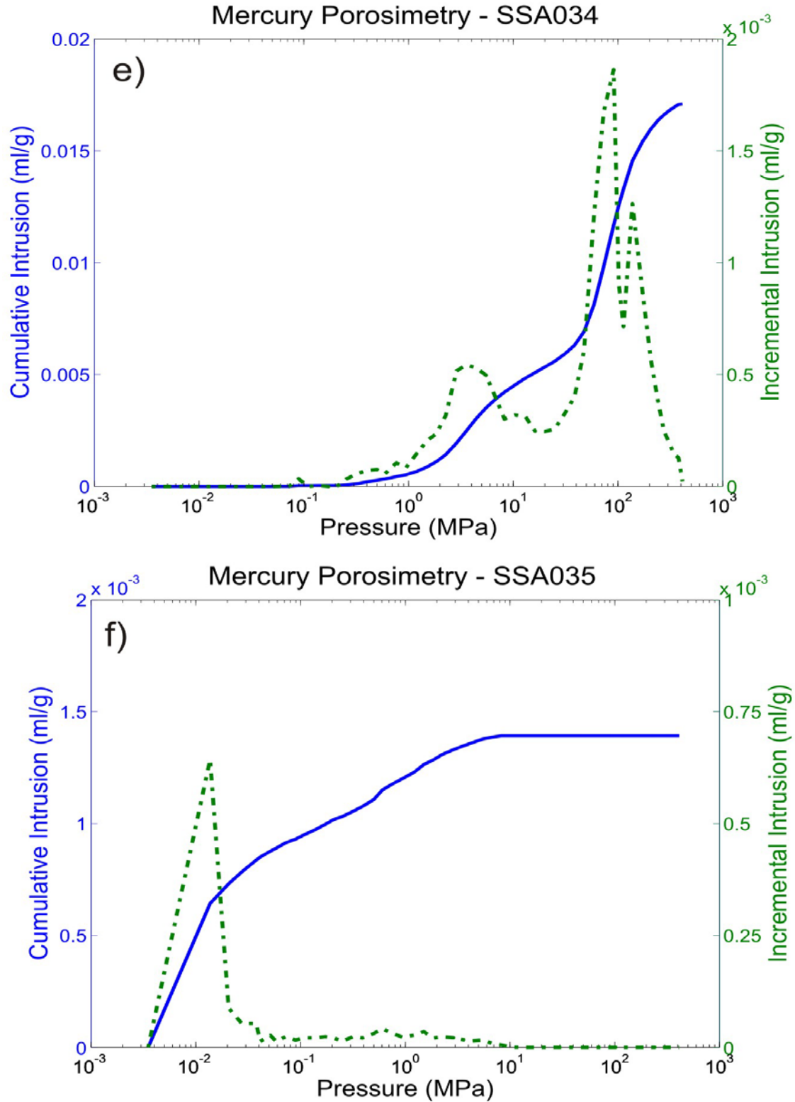
Figure 4.4 ( continued ) - Cumulative and incremental intrusion curves for the e) 2 nd White Specks sandstone (SSA034) and f) Big Valley anhydrite (SSA035).
