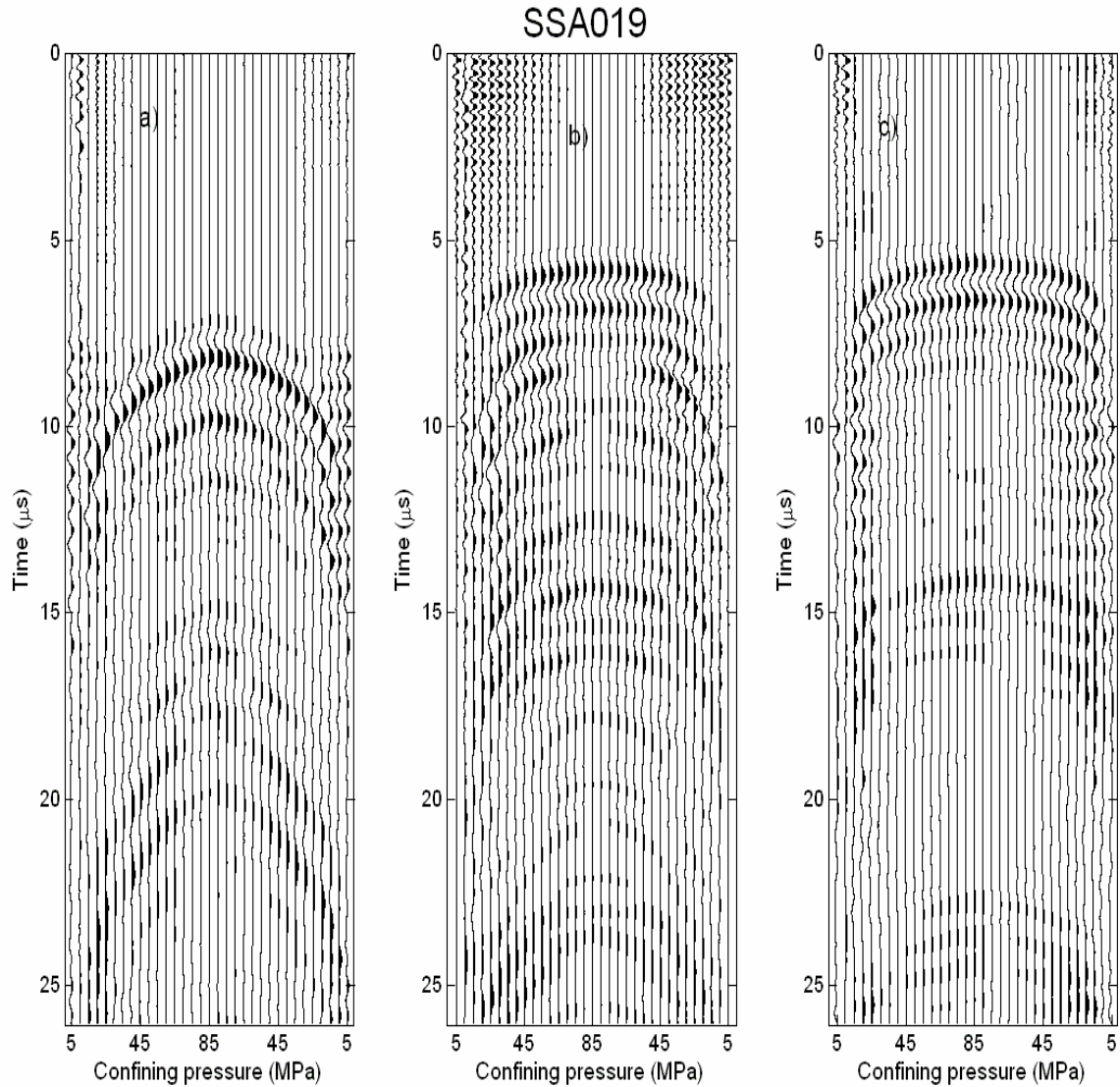
Figure 3.8 - P-waves measured in the directions a) parallel, b) 45°, and c) perpendicular to bedding in the Mount Head carbonate. This sample shows a strong dependence on travel time with pressure.
