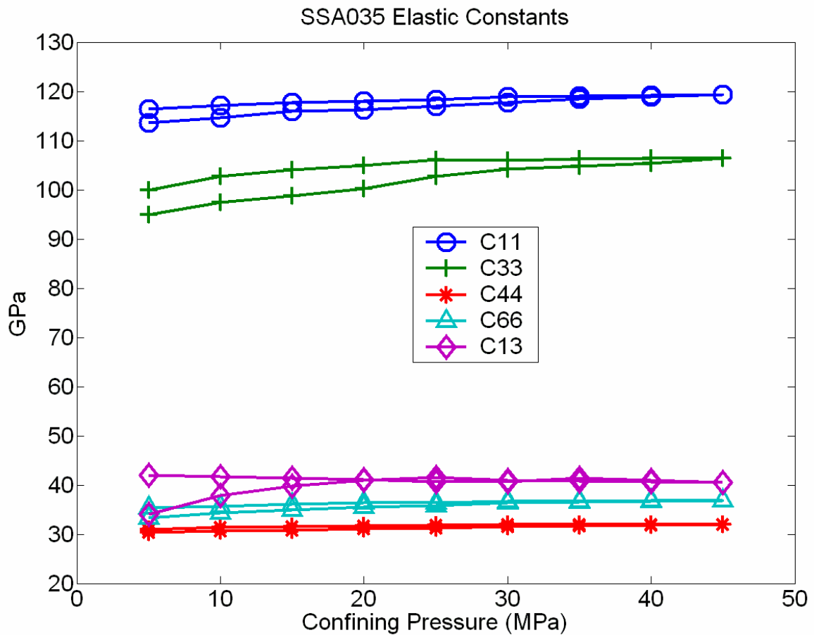
Figure A.23 - Elastic constants for the Big Valley anhydrite.
