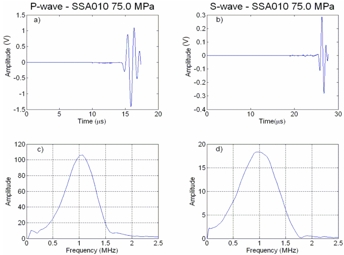
Figure 3.10 - a) The initial signal and c) amplitude spectrum of P-waves through the Mannville shale 1. The same is shown for S-waves in b) and d). The peak frequency is near 1 MHz.
