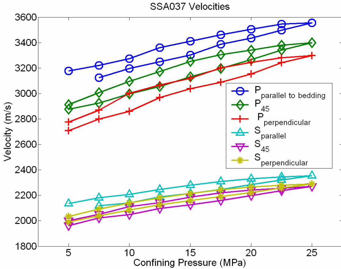
Figure A.26 - Velocities for the Bow Island sandstone.
