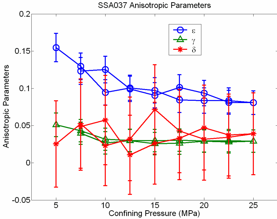
Figure A.28 - Anisotropic parameters of the Bow Island sandstone.
