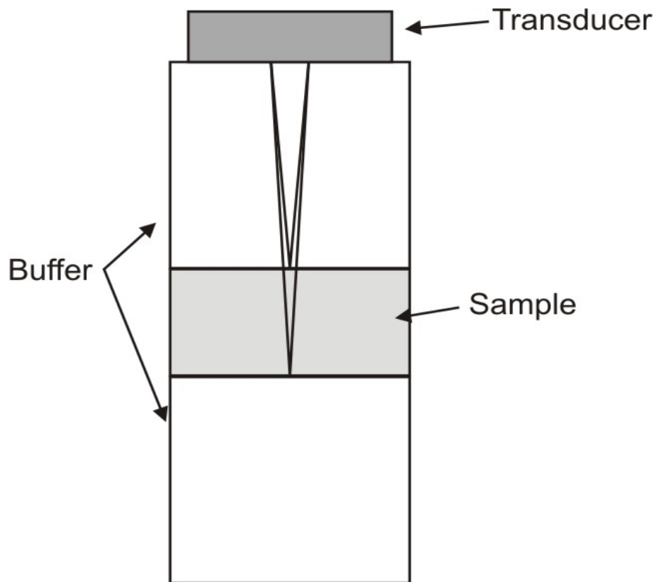
Figure 2.7 - The basic premise of a pulse reflection experiment. A pulse is reflected from the top and bottom of the sample. The difference in times is used to calculate the velocity.
