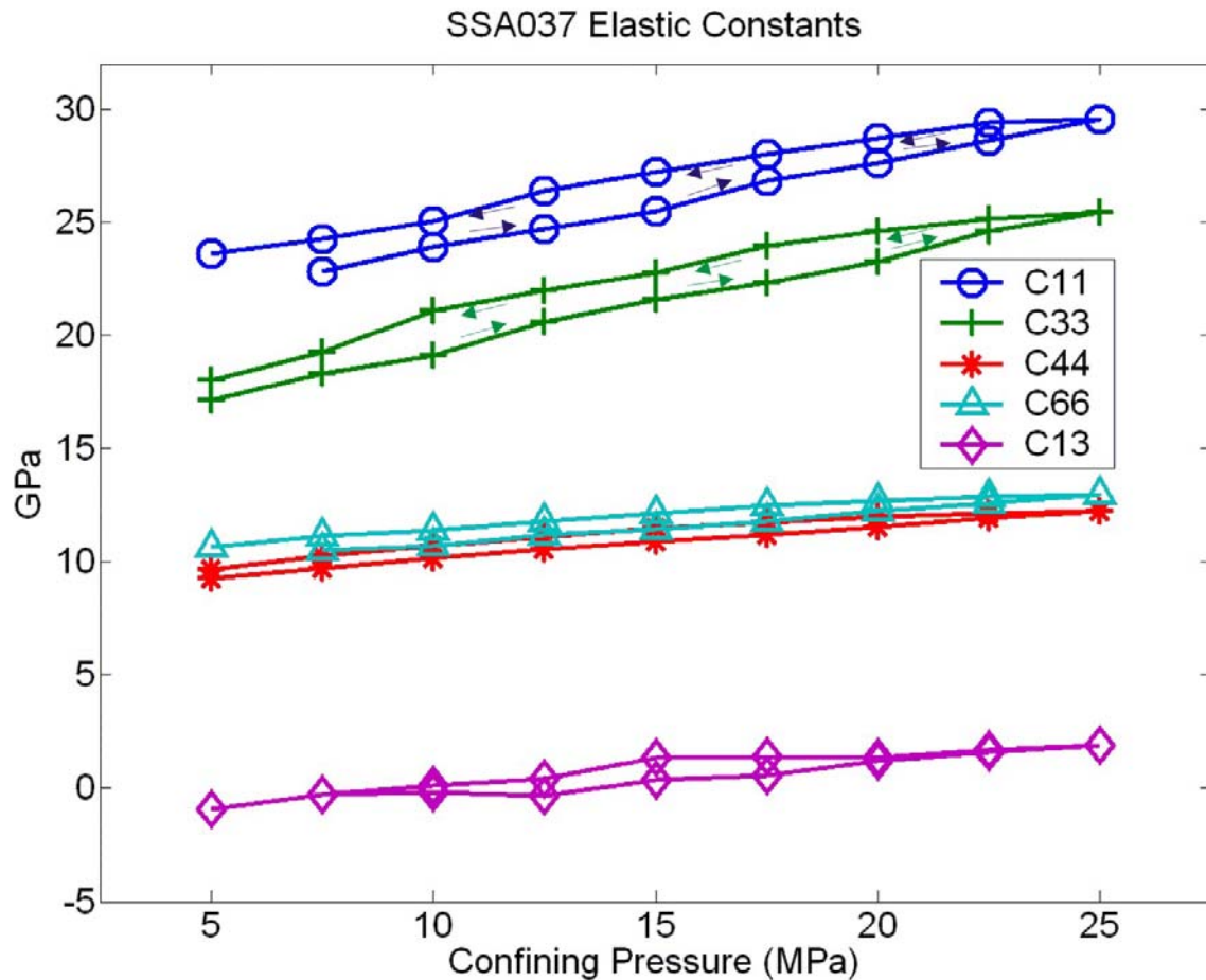
Figure 5.10 - Elastic constants for the Bow Island sandstone. Hysteresis effects cause the values to be higher during depressurization. Progression is indicated by arrows on C_{11} and C_{33} , and omitted on the other elastic constants for clarity.
