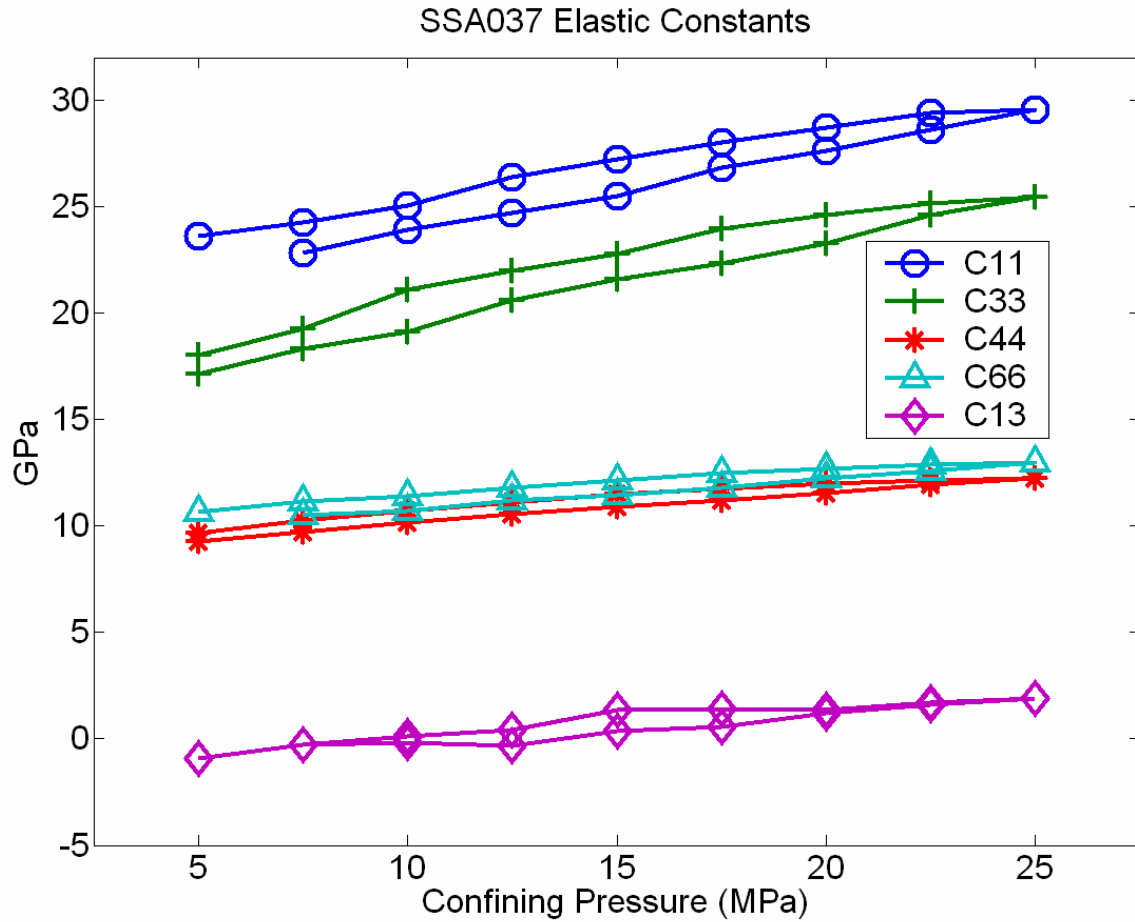
Figure A.27 - Elastic constants for the Bow Island sandstone.
