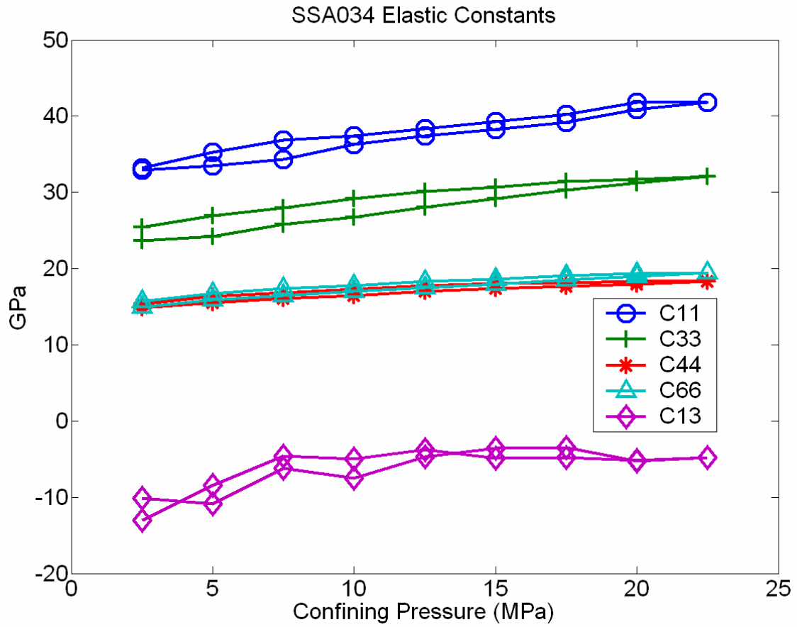
Figure A.19 - Elastic constants of the 2 nd White Specks sandstone.
