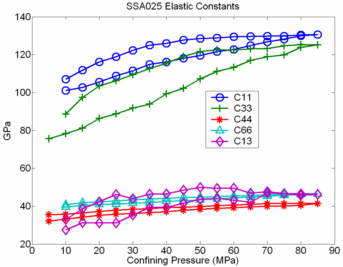
Figure A.15 - Elastic constants for the Wabamun carbonate.
