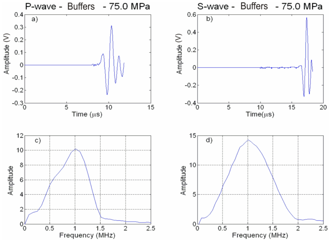
Figure 3.9 – a) The initial signal and c) amplitude spectrum of P-waves through the buffers. The same is shown for S-waves in b) and d). The peak frequency is around 1 MHz in both the P- and S-waves.
