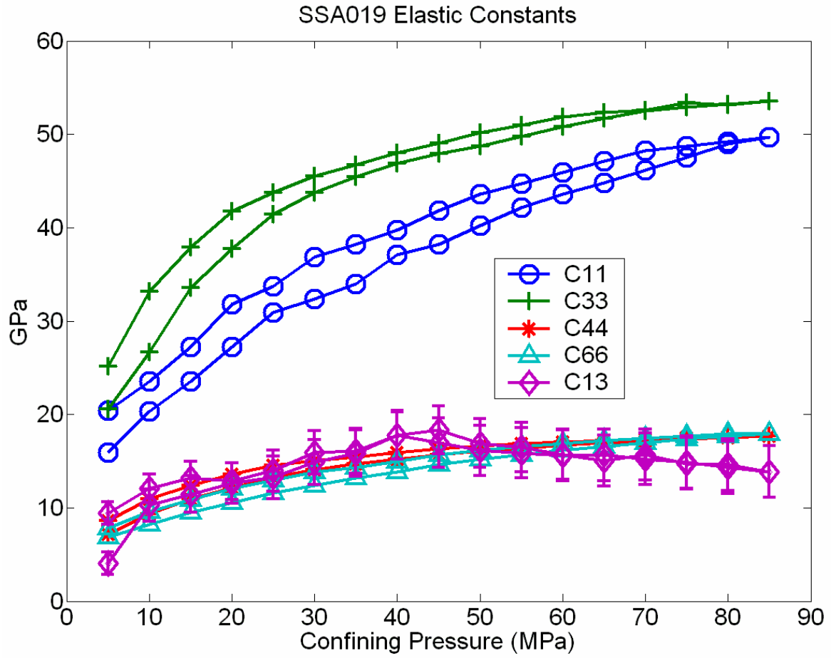
Figure A.11 - Elastic constants of the Mount Head carbonate.
