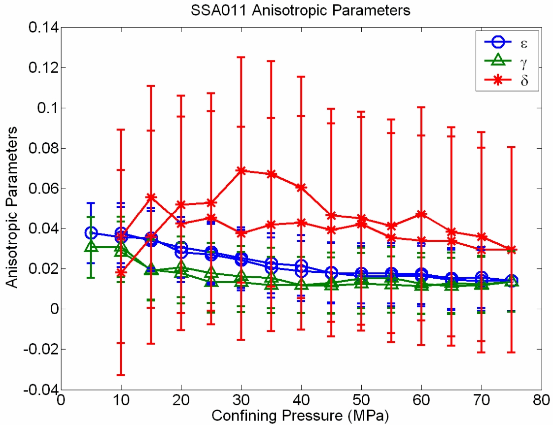
Figure A.8 - Anisotropic parameters of the Mannville shale 2.
