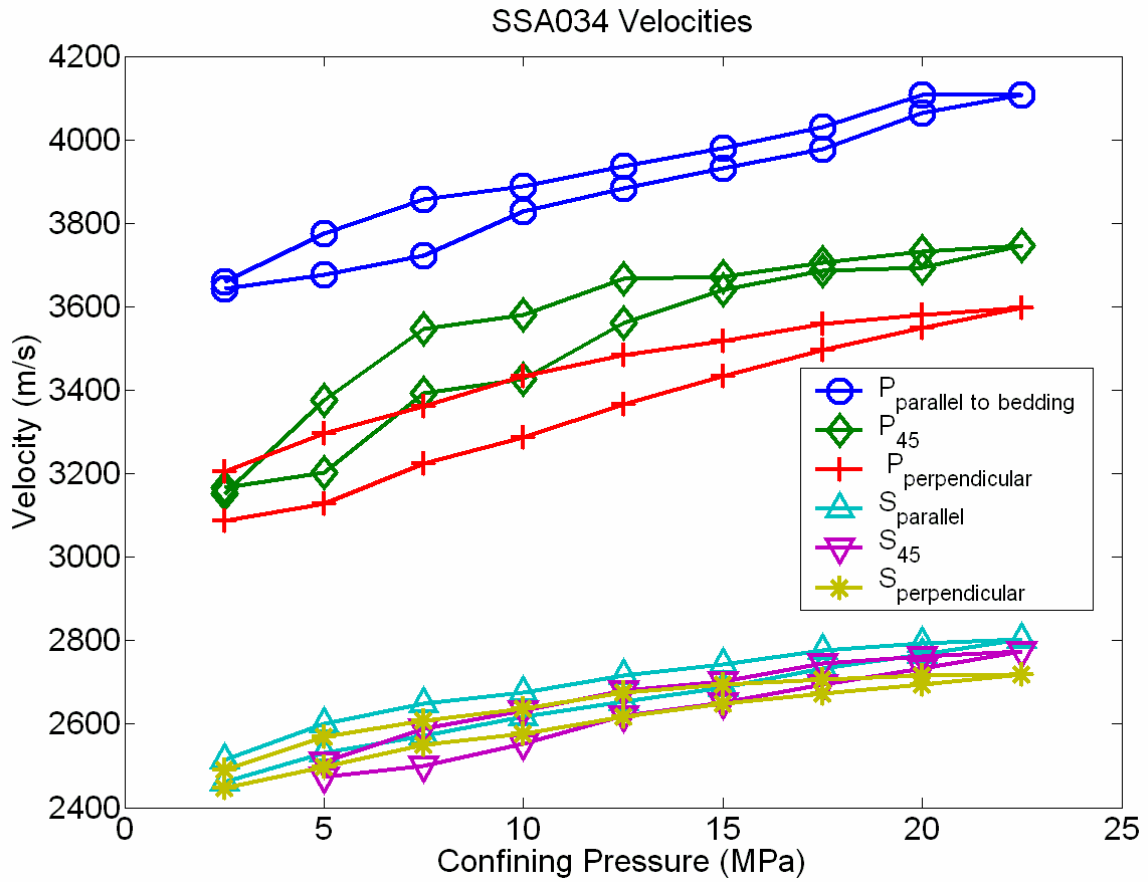
Figure A.18 - Velocities for the 2 nd White Specks sandstone.
