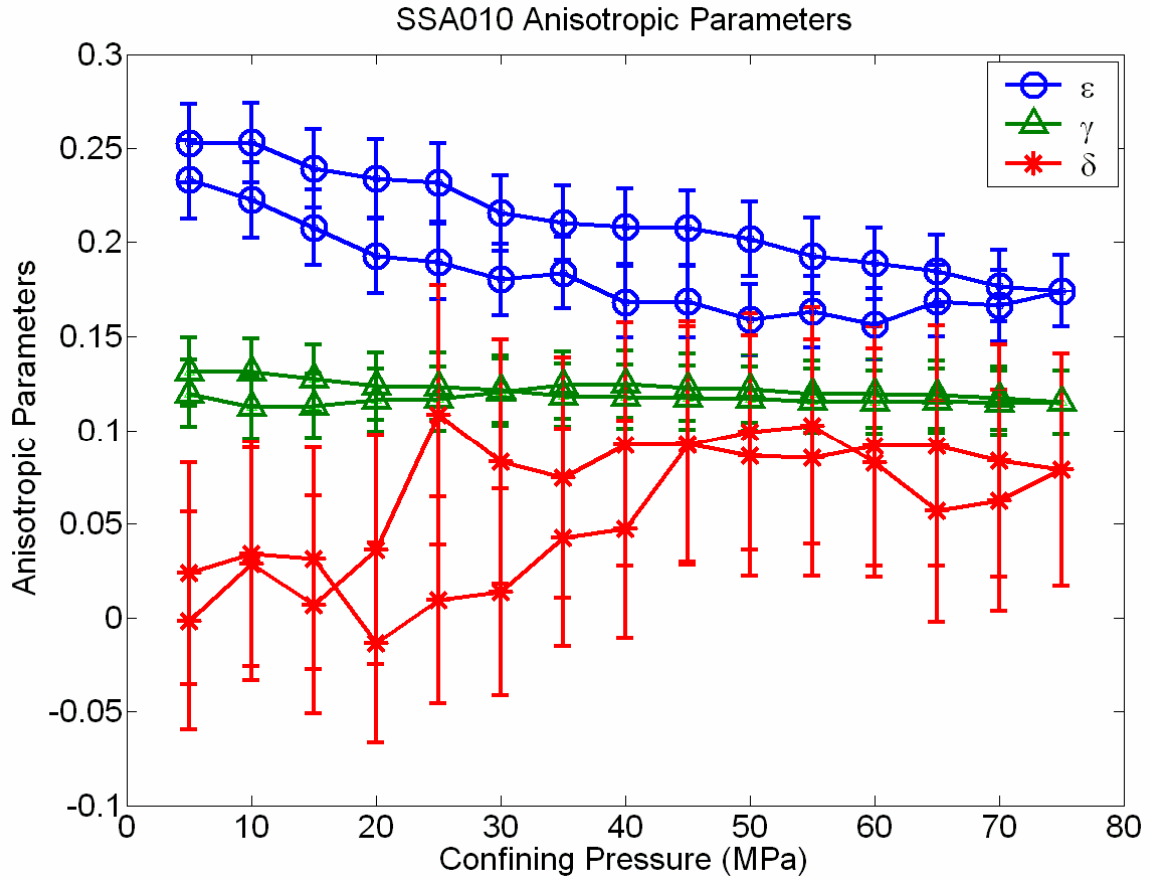
Figure A.4 - Anisotropic parameters of the Mannville shale 1.
