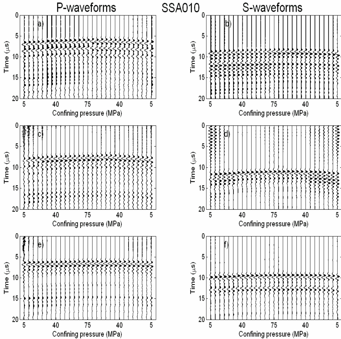
Figure 3.7 – Complete suite of waveforms obtained for the Mannville shale 1. a) and b) show the P- and S-waves, respectively, traveling perpendicular to bedding. c) and d) show the waveforms traveling 45 to bedding, and e) and f) show the waveforms parallel to bedding.
