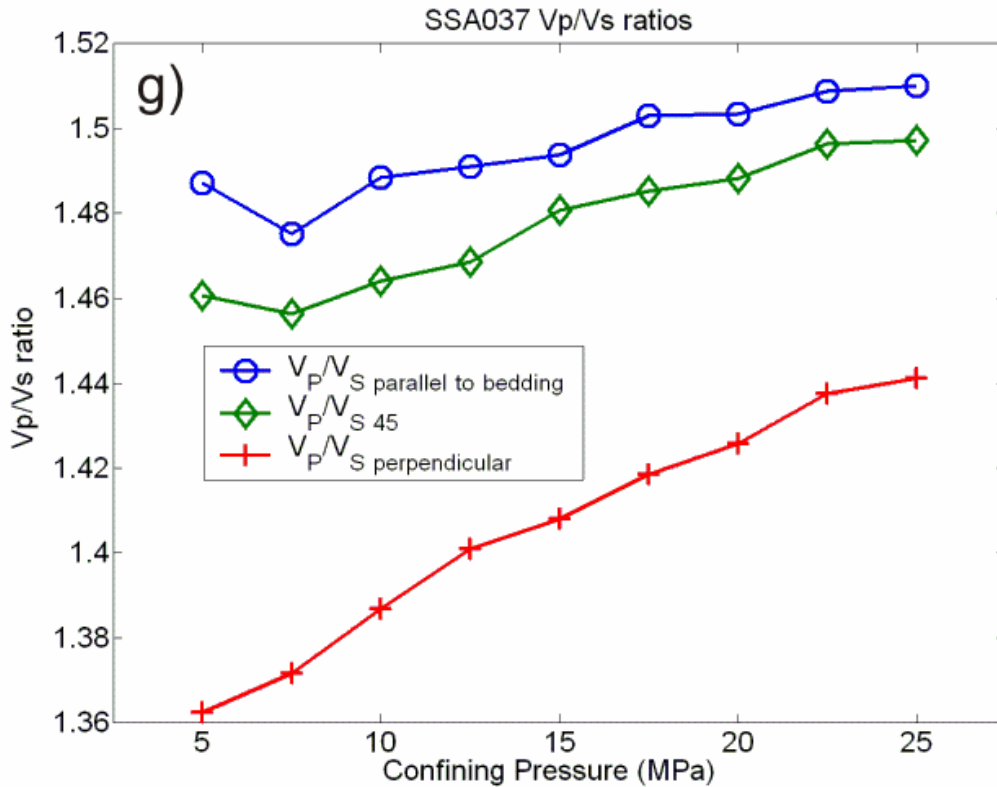
Figure 5.13 (continued) - V_P/V_S ratios for g) the Bow Island sandstone (SSA037).
