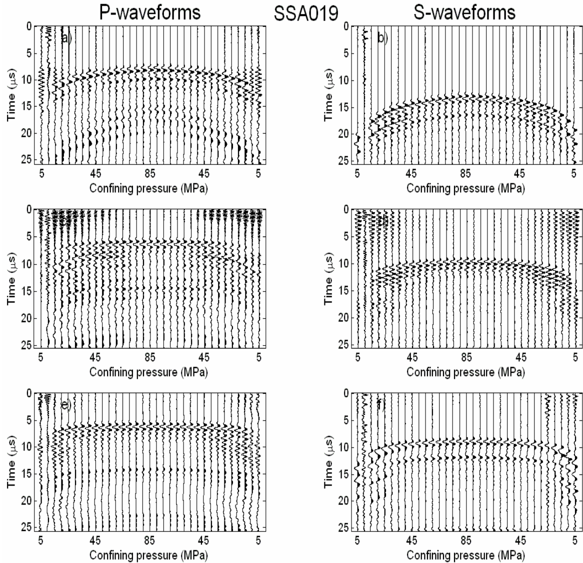
Figure A.9 – Complete suite of waveforms obtained for the Mount Head carbonate. a) and b) show the P- and S-waves, respectively, traveling perpendicular to bedding. c) and d) show the waveforms traveling 45° to bedding, and e) and f) show the waveforms parallel to bedding.
