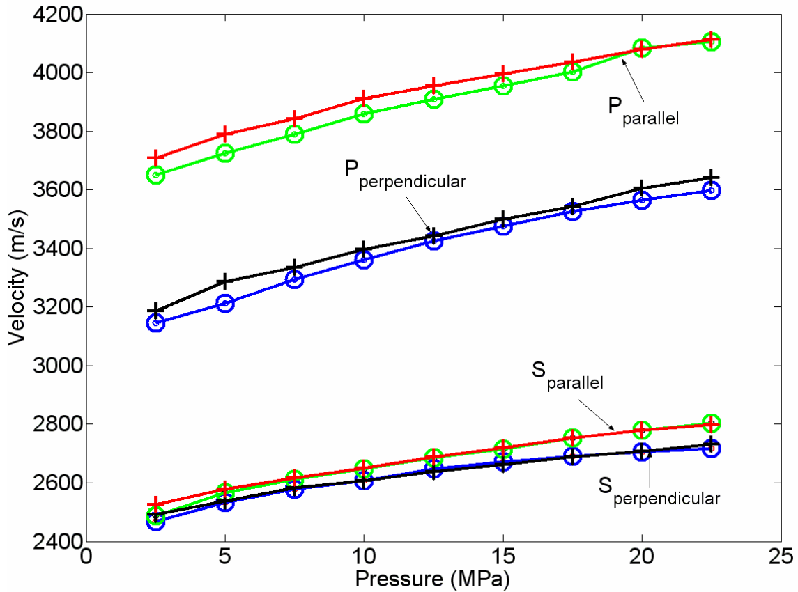
Figure 5.1 - Results of consolidation tests on the 2 nd White Specks sandstone. The first test is represented by blue and green 'o' markers, while the second test is indicated by black and red '+' markers.
