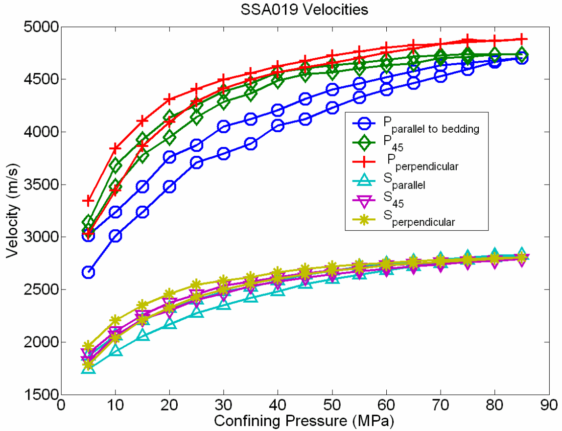
Figure A.10 - Velocities for the Mount Head carbonate.
