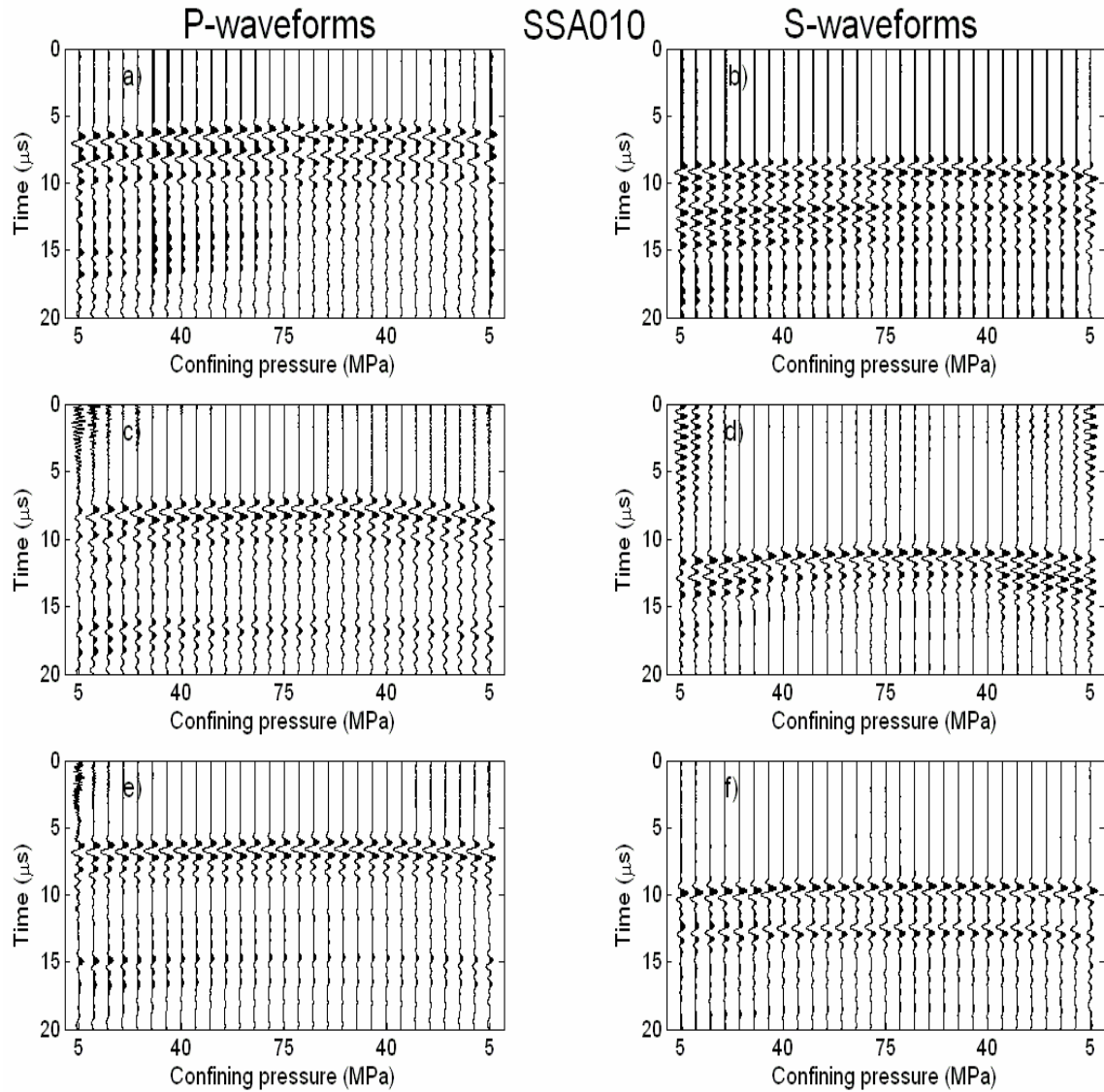
Figure A.1 – Complete suite of waveforms obtained for the Mannville shale 1. a) and b) show the P- and S-waves, respectively, traveling perpendicular to bedding. c) and d) show the waveforms traveling 45^\circ to bedding, and e) and f) show the waveforms parallel to bedding.
