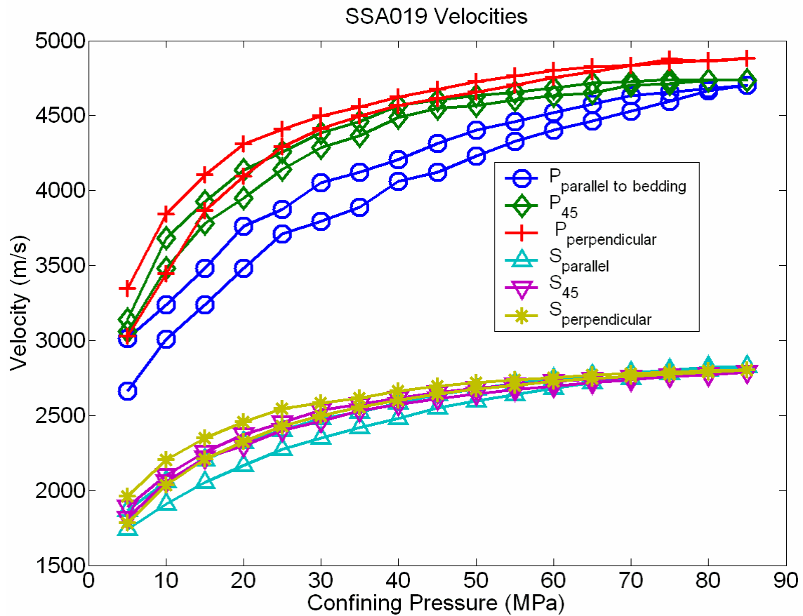
Figure 5.3 - Velocities of the Mount Head carbonate. Each velocity is measured for increasing and decreasing pressure. Velocities are higher for decreasing pressure.
