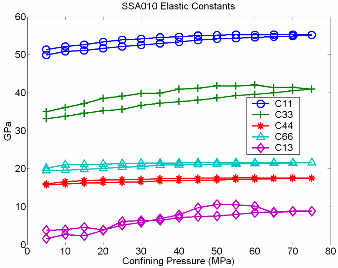
Figure A.3 - Elastic constants for the Mannville shale 1. Lower curve is increasing pressure and upper curve is decreasing pressure.
