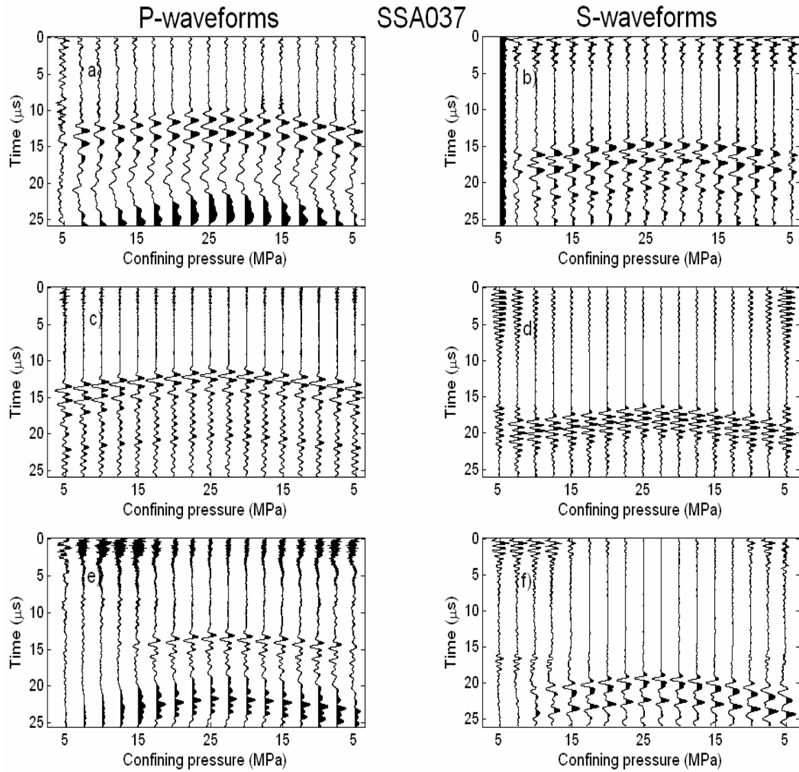
Figure A.25 – Complete suite of waveforms obtained for the Bow Island sandstone. a) and b) show the P- and S-waves, respectively, traveling perpendicular to bedding. c) and d) show the waveforms traveling 45^\circ to bedding, and e) and f) show the waveforms parallel to bedding.
