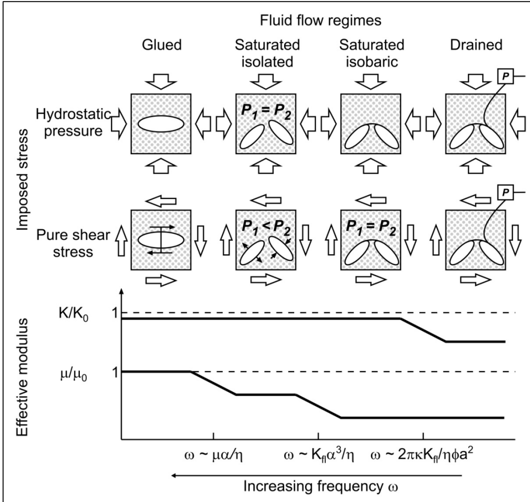
Figure 2.1: Fluid-flow regimes and effective elastic moduli for cracked, fluid saturated rocks (O'Connell and Budiansky, 1977), after Jackson (1991) with permission. The upper panels show the response of the crack to hydrostatic (top row) and shear (second row) pressure, while the lower graphs show the expected bulk and shear modulus behaviour in each regime as a function of angular frequency, \omega . P_1 and P_2 are the pore pressures in the cracks, with their relationship depending on fluid flow regime and crack orientation.
