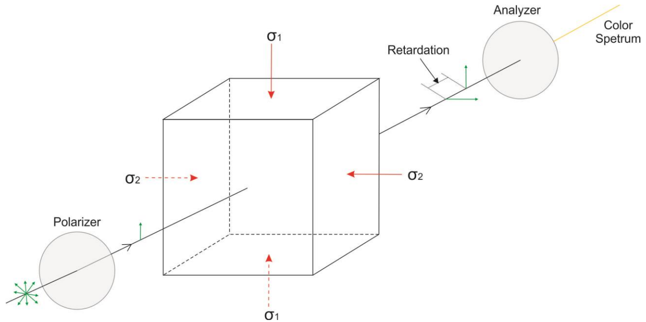
Figure A.3 Transmission of a beam of natural light in the photoelasticity experimental setup. Green arrows indicate polarization directions of light. Polarizer is the first polarizing filter that the light encounters forming in a beam of polarized light. The cube represents an optical sample with stress birefringent effects. After traveling through the sample, the light is separated into two beams of polarized light with different speeds. Upon rotating the second polarizing filter, also known as the analyzer, we can control the appearance of the color spectrum.
