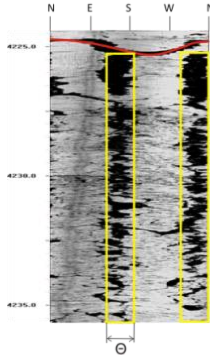
Figure 3.3 Borehole televiewer image data from southern Idaho shows a planar feature (red line) and borehole breakouts (yellow boxes). Based on a work that is done by ( Shervais et al. , 2013).
