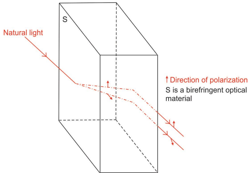
Figure A.2 A beam of natural light separates into two beams with different polarizations and velocities when traveling through a birefringent material. Their polarizations are orthogonal to each other, along directions of the principal axes of the optical material. Modified from Chartier (2005).
