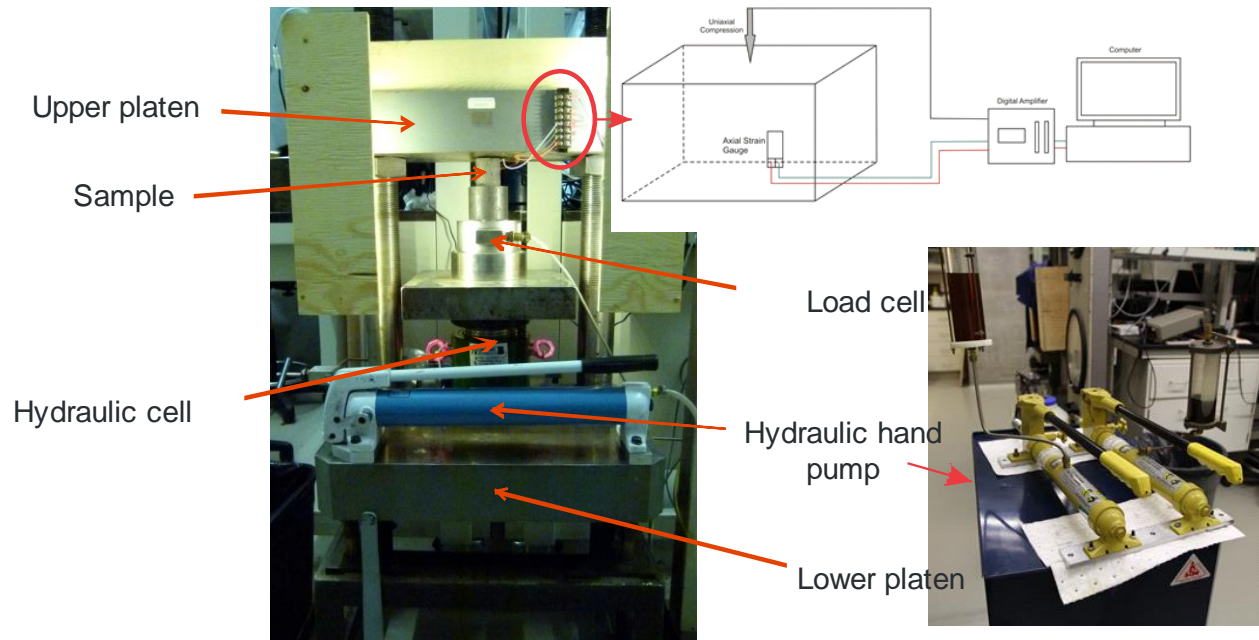
Figure 3.7 The experimental setup. The cartoon in the upper right shows the configuration of the data transmission and recording systems. The sample was placed in between the upper platen and the load cell. Pressures were applied on the double hydraulic hand pump and then transferred through the hydraulic system.
