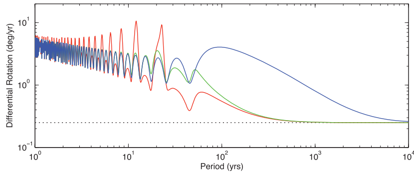
Figure 4. Amplitudes of inner core differential rotation for a forcing applied to the tangent cylinder subject to the constraint that LOD changes do not exceed 3 ms in amplitude at the given period. Three different sets of gravitational coupling parameters are shown: \bar{\Gamma} = 3 \times 10^{20} N m and \tau = 0.166 yr (red line); \bar{\Gamma} = 5 \times 10^{18} N m and \tau = 10 yr (green line); \bar{\Gamma} = 1 \times 10^{17} N m and \tau = 500 yr (blue line). Other parameters are as given in Table 1. The dotted horizontal lines indicate an inner core super-rotation of 0.25^\circ \text{ yr}^{-1} .
