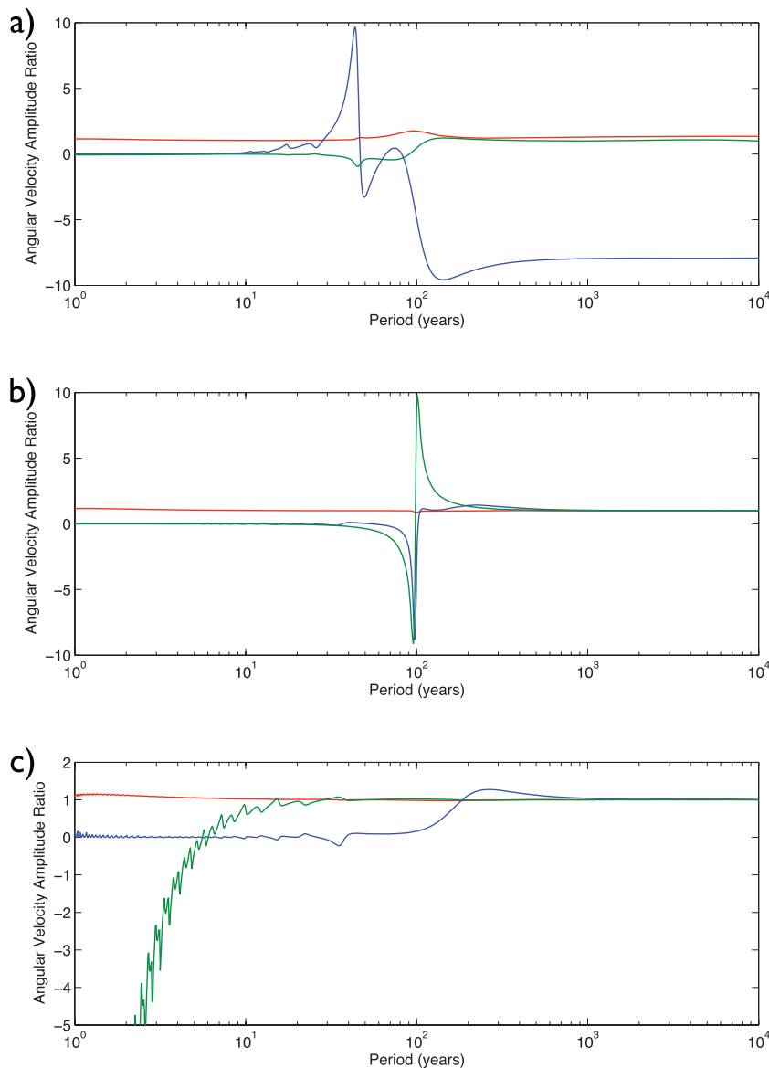
Figure 1. Angular velocities relative to that of the inner core for a forcing applied to the (a) tangent cylinder (b) inner core and (c) mantle. All panels show the velocities of the fluid inside the tangent cylinder (red lines), the fluid outside the tangent cylinder (blue lines) and the mantle (green lines). The viscous relaxation time of the inner core is \tau = 1000 yr, all other parameters are as given in Table 1.
