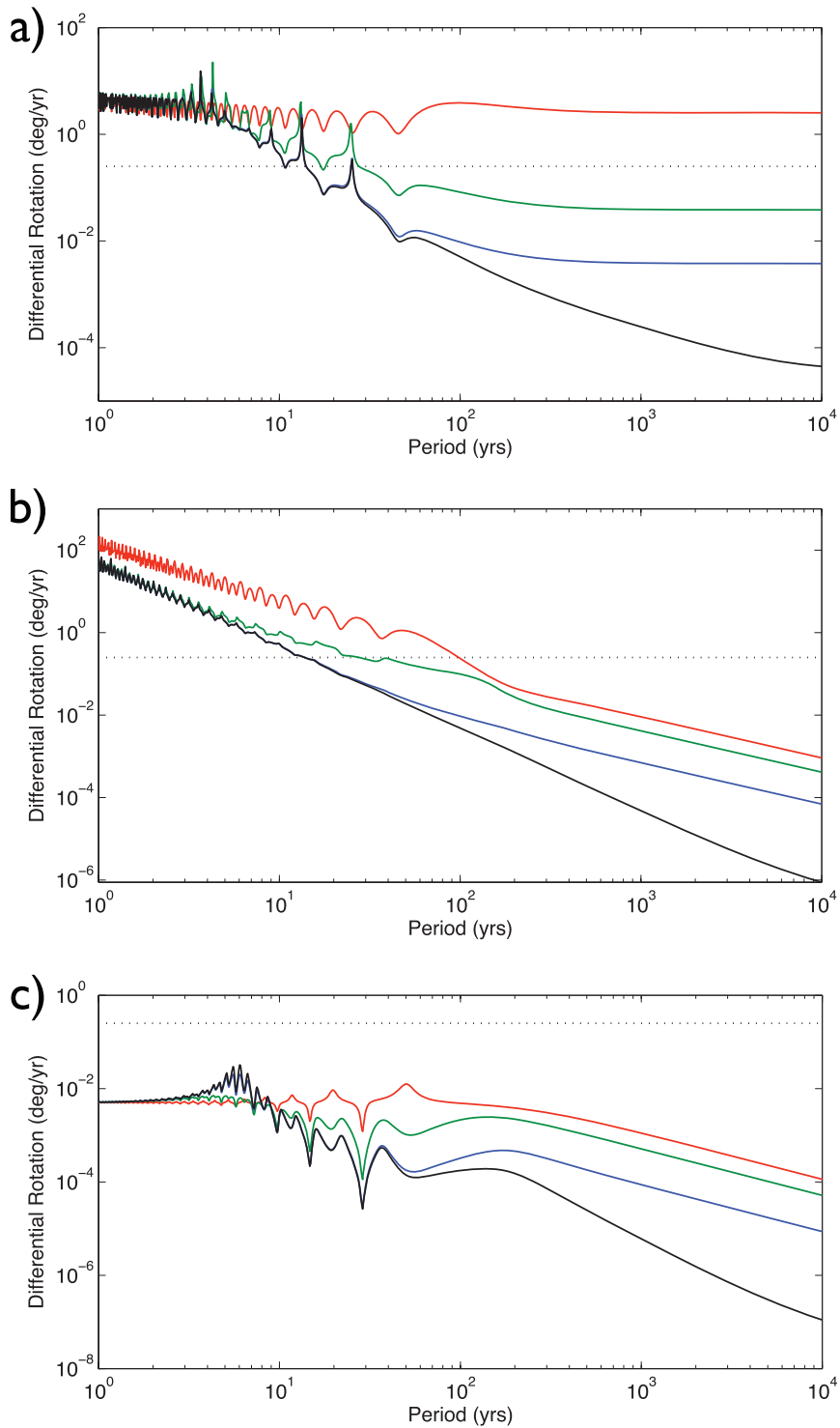
Figure 3. Amplitudes of inner core differential rotation for oscillatory motion subject to the constraint that LOD changes do not exceed 3 ms in amplitude at the given period. We consider models with no gravitational coupling (red lines), and gravitational coupling with an inner core relaxation time of 1 yr (green lines), 10 yr (blue lines) or 1000 yr (black lines). The dotted horizontal lines indicate an inner core differential rotation of 0.25^\circ \text{ yr}^{-1} . As in previous figures, we consider a forcing applied to the (a) tangent cylinder (b) inner core and (c) mantle.
