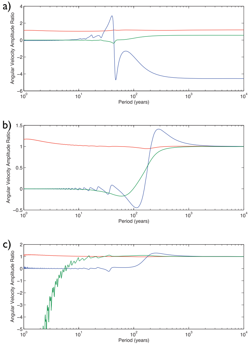
Figure 2. Angular velocities relative to that of the inner core for a forcing applied to the (a) tangent cylinder (b) inner core and (c) mantle. All panels show the velocities of the fluid inside the tangent cylinder (red lines), the fluid outside the tangent cylinder (blue lines) and the mantle (green lines). The viscous relaxation time of the inner core is \tau = 10 yr, all other parameters are as given in Table 1.
