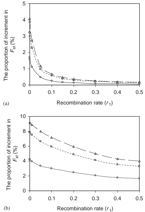
Fig. 3. The proportion of increment in F_{st} due to background selection: (a) two-locus case, with the selection coefficient s_{1i} = 0.02 ( i = 1, \dots, 30 ), the mutation rate u_1 = 10^{-5} for the A locus and v = 5 \times 10^{-4} for the C locus, the conditional probabilities in migrants \bar{x}_0 = 0.8 and \bar{x}_1 = 0.2 , the migrant gamete frequencies \bar{P}_{AC} = 0.76 and \bar{P}_{aC} = 0.01 , the migrant allele frequencies \bar{p}_A = 0.95 and \bar{p}_C = 0.8 , and the effective population size N_e = 50 ; (b) three-locus case, with the mutation rate u_1 = u_2 = 10^{-5} and v = 5 \times 10^{-4} , the selection coefficients s_{1i} = s_{2i} = 0.02 ( i = 1, \dots, 30 ), the recombination rates between the A and C loci or the B and C loci r_1 = r_2 and between the A and B loci r = 2r_1 , the LD between the A and B loci in migrants \bar{D}_{AB} = 0.03 , the migrant allele frequencies \bar{p}_A = \bar{p}_B = 0.95 , the conditional probabilities in migrants \bar{y}_0 = 0.82 , \bar{y}_1 = \bar{y}_2 = 0.7 , and \bar{y}_3 = 0.2 , and the effective population size N_e = 50 . In each figure the line with circles represents the case of \tilde{m} = 0.015 ( m_S = m_P = 0.01 ), the line with blocks for \tilde{m} = 0.05 ( m_S = 0.04 , m_P = 0.02 ), and the line with triangles for \tilde{m} = 0.10 ( m_S = 0.05 , m_P = 0.1 ).
