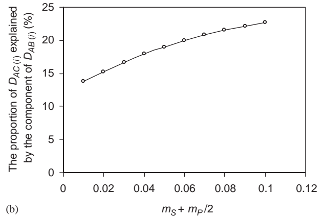
Fig. 1. Effects of the dependence between the selected A and B loci: (a) Changes in D_{AC(i)} and D_{AB(i)} with the migration rate. (b) The proportion of D_{AC(i)} explained by the component of D_{AB(i)} . D_{AB(i)} is calculated according to Eqs. (7) and (8) while D_{AC(i)} is calculated according to Eq. (11a). The settings of other parameters are the mutation rate for the A and B loci u_1 = u_2 = 10^{-5} and for the neutral locus v = 10^{-4} , the selection coefficients s_{1i} = s_{2i} = 0.02 , the recombination rates between the A and C loci or the B and C loci r_1 = r_2 = 0.01 and between the A and B loci r = 2r_1 , the LD between the A and B loci in migrants \bar{D}_{AB} = 0.03 , the migrant allele frequencies \bar{p}_A = \bar{p}_B = 0.8 , and the conditional probabilities in migrants for the neutral locus C under different backgrounds \bar{y}_0 = 0.8 , \bar{y}_1 = \bar{y}_2 = 0.7 , and \bar{y}_3 = 0.2 .
