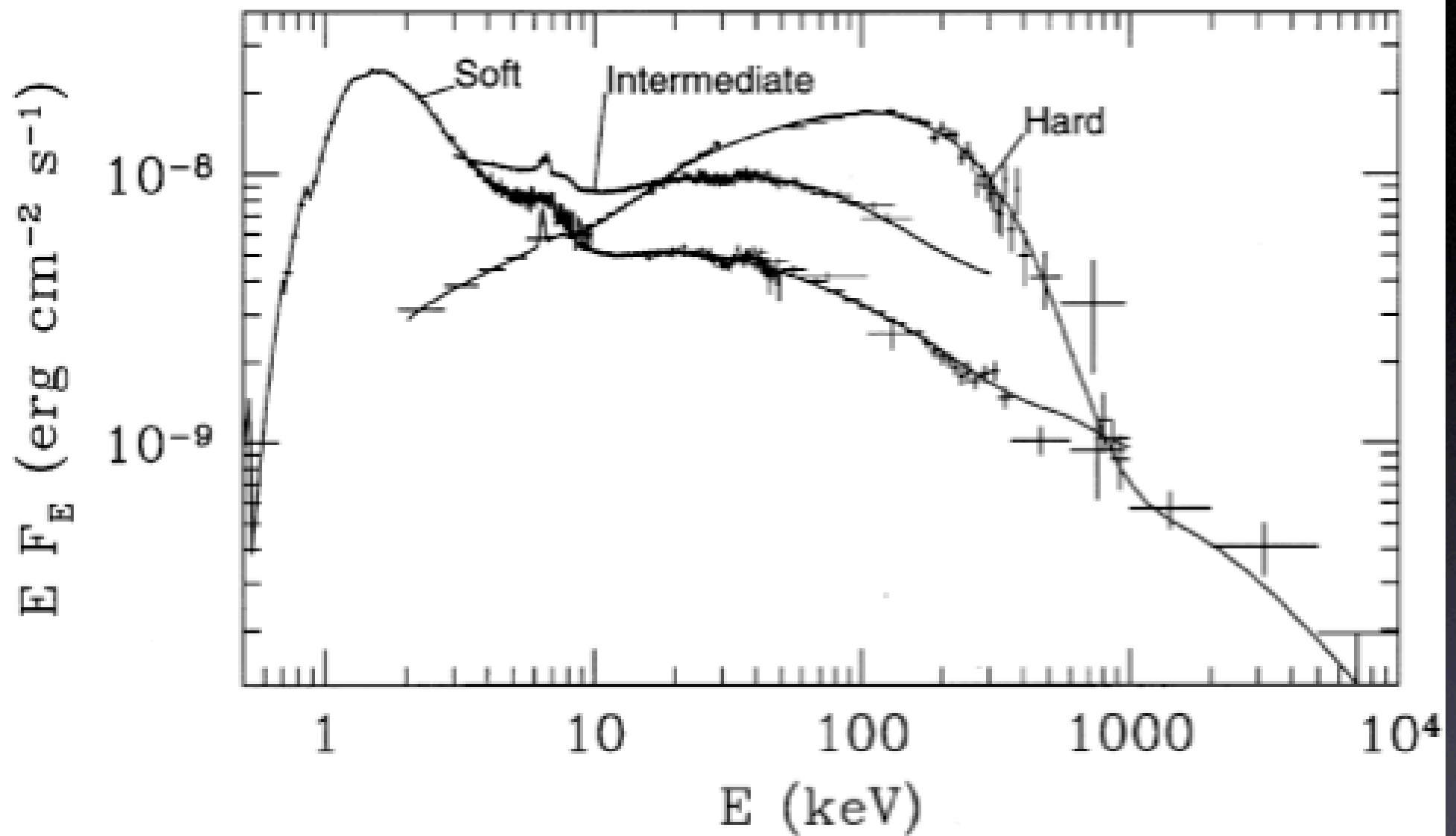
X-ray Spectra of Cygnus X-1
