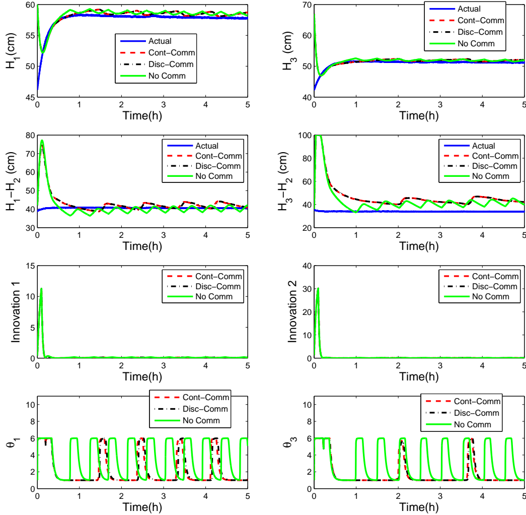
Figure 6.7: Trajectories of the levels, interactions and innovations in DAHGKF with continuous, discrete and absence of communication for the first and third subsystems.
