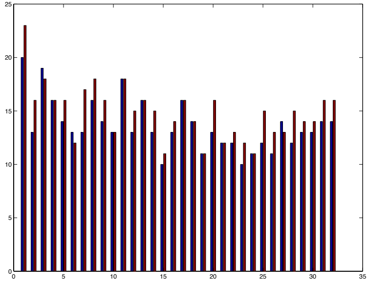
Figure 5.3: Numbers of iterations given by prediction-driven CDMHE (right side) and prediction-driven CDMHE with triggered communication (left side) during each sampling time k .
