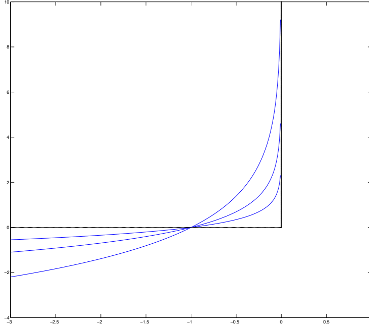
Figure 4.2: The dashed lines show the function \rho_-(u) and the solid lines show \hat{\rho}_-(u) = -(1/t)\log(-u) .
