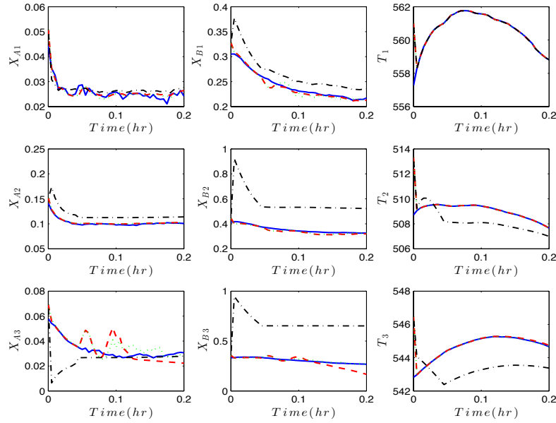
Figure 5.8: Communication Failure Case 2: State trajectories of the actual state (solid line), estimated states given by the proposed CDMHE (dashed line), the centralized MHE (dotted line), and the decentralized MHE (dash-dotted line).
