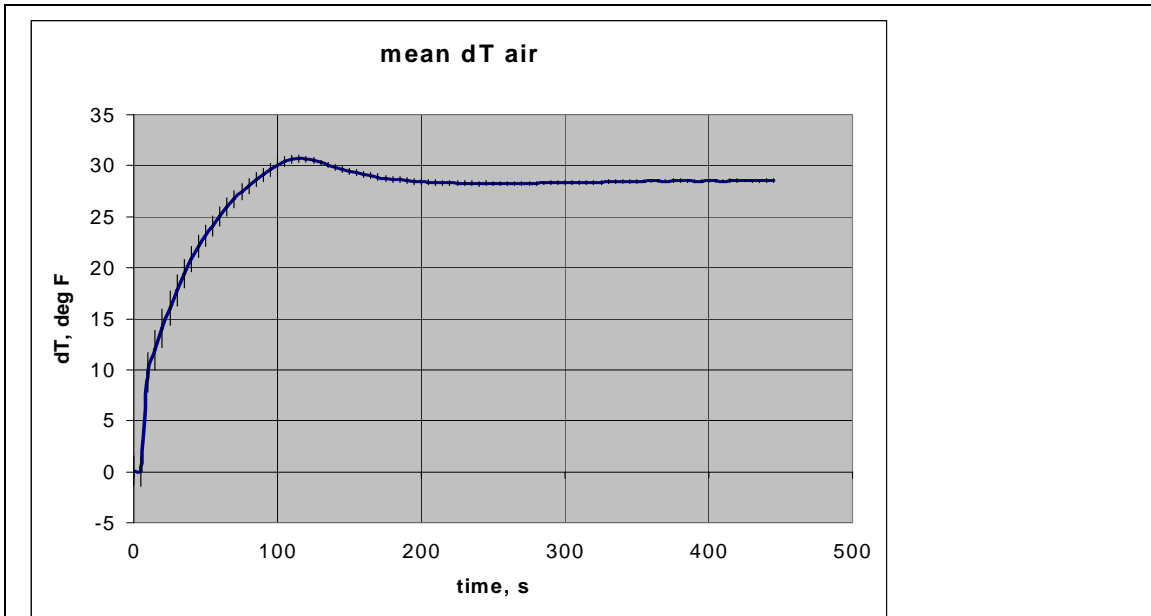
Fig. 4: dT = (\text{Temp air out} - \text{Temp air in}) . Time 0 = 10 s before power supplied to the compressor. Line gives mean trend without points. Vertical bars are standard deviations at 5 s intervals. N = 451 .
