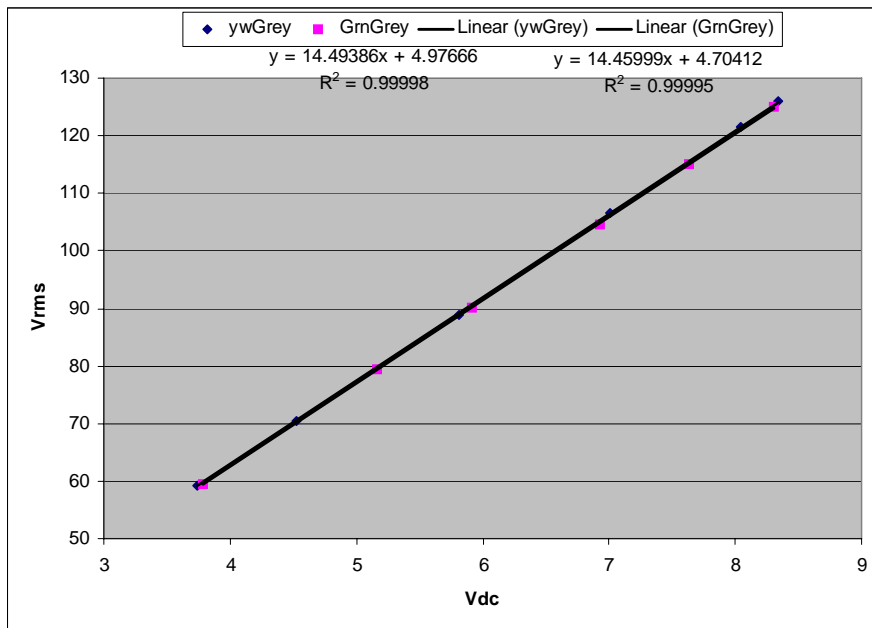
Fig. 2: Typical calibration of my custom-built sensor for converting V_{\text{RMS}} to V DC. The normal operating range is 110 to 120 V AC @ 60 Hz
