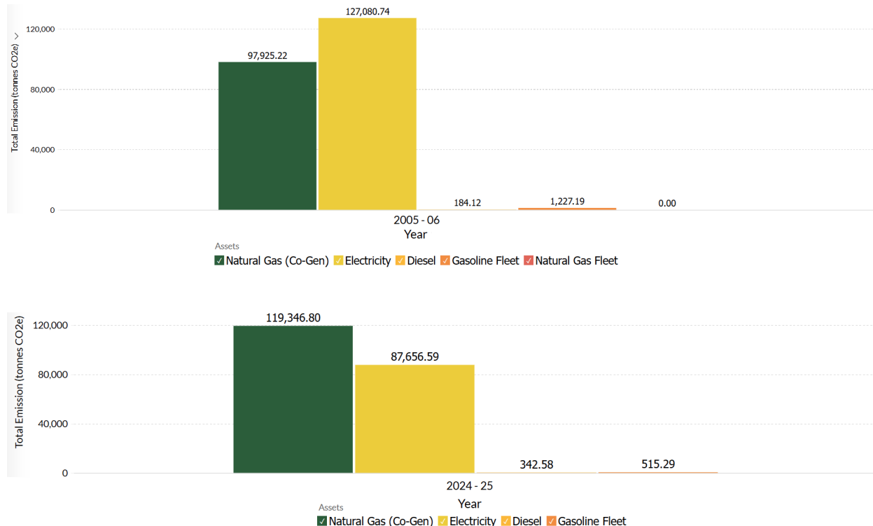
Figure 2-7. Summary of U of A emissions in the base year of 2005/06 and reporting year of 2024/25, broken down by fuel source.
