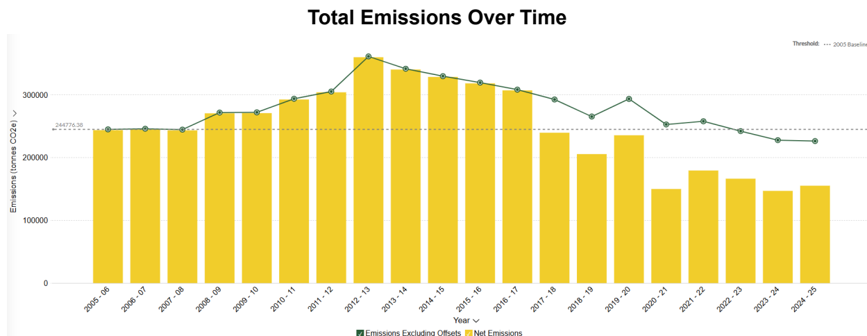
Figure 2-8. Total emissions over time starting with the base year of 2005/06 until the 2024/25 reporting year. Net emissions met and surpassed the goal to reduce emissions by 17% below the 2005/06 threshold.
