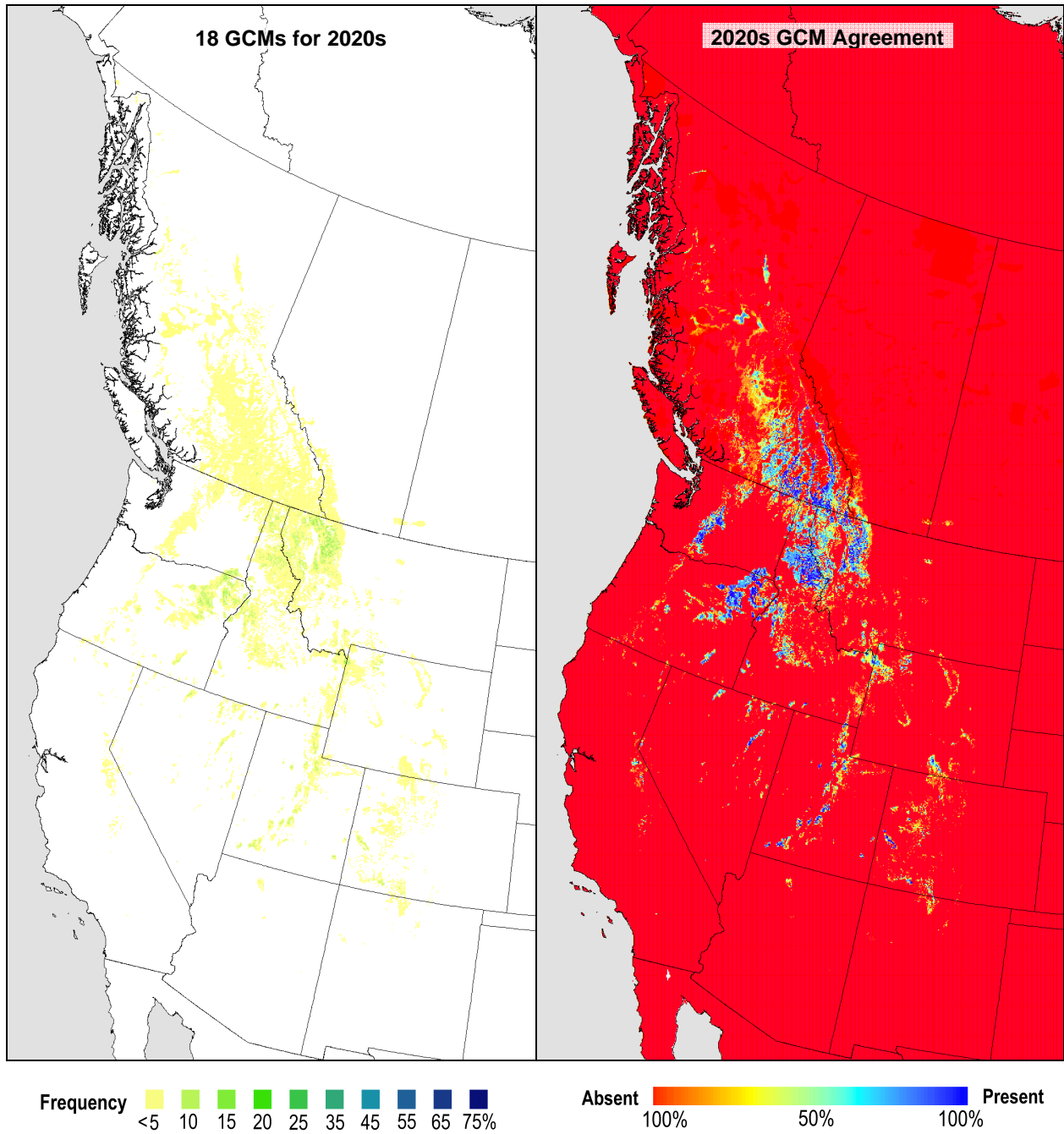
Figure S11b. Projected habitat of western larch for the 2011–2040 normal period according to 18 climate change projections. The left image is an average expected frequency (% canopy cover projected to the ground). The right image represents agreement of species presence/absence projections for 18 general circulation models.
