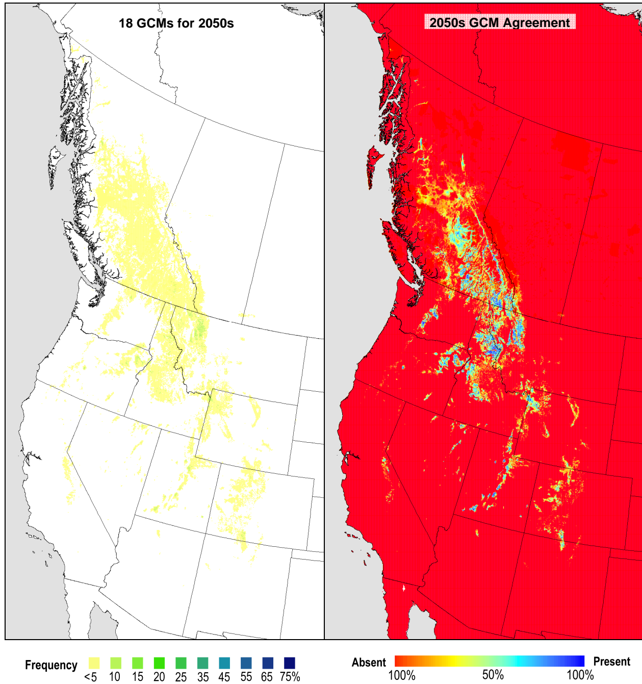
Figure S11c. Projected habitat of western larch for the 2041–2070 normal period according to 18 climate change projections. The left image is an average expected frequency (% canopy cover projected to the ground). The right image represents agreement of species presence/absence projections for 18 general circulation models.
