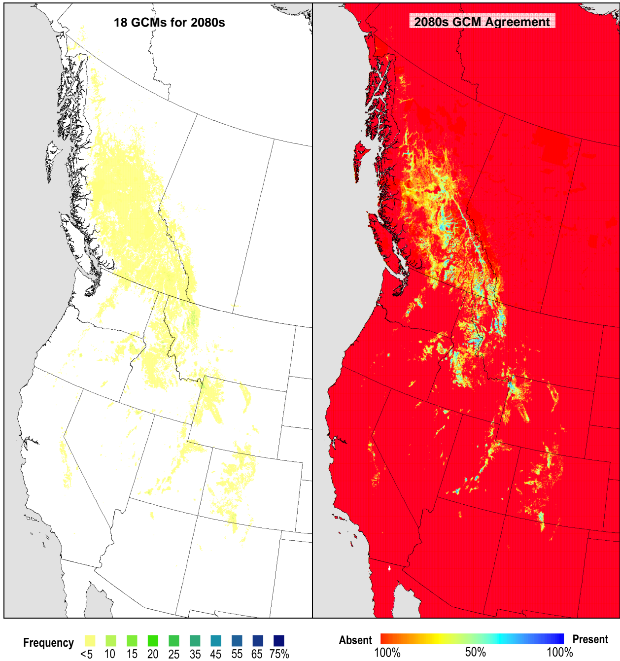
Figure S11d. Projected habitat of western larch for the 2071–2100 normal period according to 18 climate change projections. The left image is an average expected frequency (% canopy cover projected to the ground). The right image represents agreement of species presence/absence projections for 18 general circulation models.
