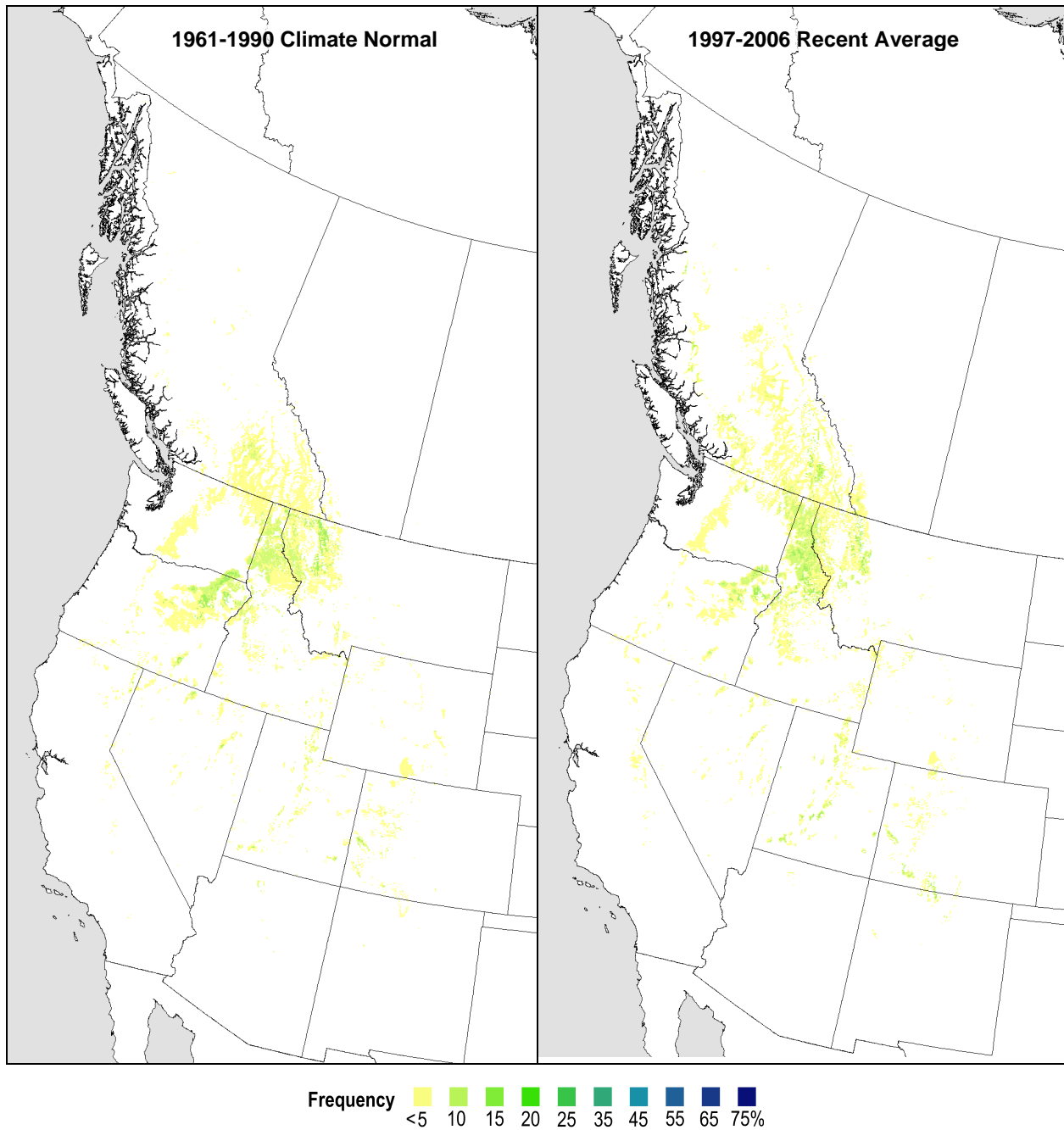
Figure S11a. Projected habitat of western larch ( Larix occidentalis Nuttall). The left image is an expected frequency (% canopy cover projected to the ground) for the 1961-1990 normal period, representing long-term climate condition and model training data. The right image models habitat for the 1997-2006 period, representing a recent (25-year) climate trend.
