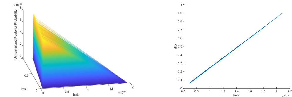
(a) Unnormalized posterior distribution over \beta - \rho space (b) A curve of most likely parameters
