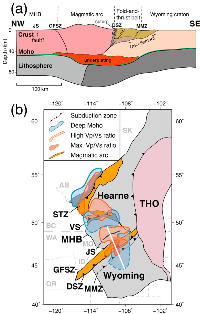
Figure 12. (a) A schematic cross-section showing the mechanisms of crustal thickening near the Great Falls Tectonic Zone (GFTZ). The location of the profile is shown by the white line in (b). The crust could be thickened by arc magmatism, arc-continent collision, load of the fold-and-thrust belts and magmatic underplating. Note that the Joplin Structure (JS), originally defined as the northern boundary of the GFTZ, does not show a significant increase in Moho depth and likely represents an intracontinental structure. (b) A map showing the Hearne-MHB-Wyoming (HMW) tectonic system, which is featured by contemporaneous (2.0–1.8 Ga) subductions, continent-continent collisions, and the associated magmatic events on the western margin of Laurentia. Superimposed regions with a deep Moho (blue contours) and high Vp/Vs ratios (red contours) are selected based on threshold values of 38 km and 1.82, respectively, near the Snowbird Tectonic Zone (STZ). The corresponding contour values near the VS and GFTZ are 40 km and 1.84, respectively. The dashed contour indicates questionable boundaries of deep Moho due to insufficient data.
