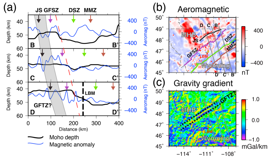
Figure 10. (a) Moho depth along three profiles that traverse the Great Falls Tectonic Zone (GFTZ). The intersections between the profiles and faults are indicated by the arrows. The shaded region indicates the location of the GFTZ defined by the gravity gradients shown in (c). The red dashed line marks the onset of crustal thickening. (b) Aeromagnetic anomalies near the GFTZ. Three sample cross-sections are marked by gray lines, and faults are delineated by thick lines in various colors. (c) Normalized gravity gradients near the GFTZ. The GFTZ is originally defined as a narrow zone between the two parallel, negative gravity gradient lineaments (dashed lines) in northern Montana (e.g., Clowes et al., 2002; Gorman et al., 2002); this definition is challenged by the results of this study.
