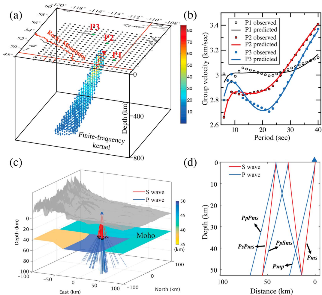
Figure 3. (a) Station-side finite-frequency kernels for shear velocity inversions, constructed using a teleseismic event at an epicentral distance of 85^\circ . The circles show the inversion nodes where dispersion curves are computed from ambient noise correlation functions (Gu & Shen, 2015). Three nodes (green circles) are selected to show the sample dispersion curves (see Figure 3b). (b) Dispersion curves from selected nodes (P1–P3). The circles mark the observed group velocities at each period and the solid lines represent the predicted dispersion curves from 1-D shear velocity inversions (Gu & Shen, 2015). (c) A schematic diagram demonstrating the ray paths of P -to- S conversions beneath a station in the foothills. The conversion points are marked by the black circles on the Moho interface. (d) Ray paths of a direct P wave and four converted phases of a teleseismic event at an epicentral distance of 45^\circ incident beneath a recording station. Compressional and shear waves are indicated using blue and red colors, respectively.
