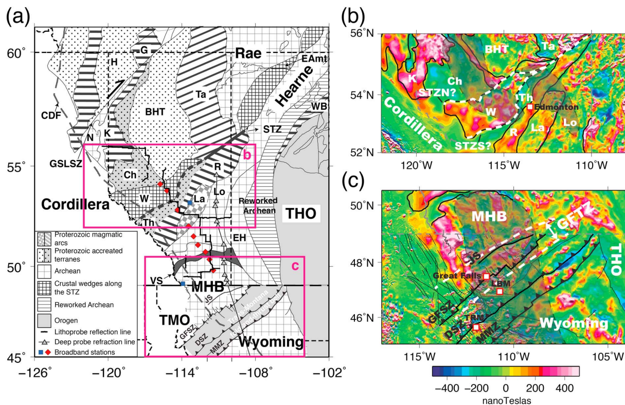
Figure 1. (a) Tectonic map of western Laurentia, modified after Ross et al. (1991). The two proposed tectonic boundaries (Snowbird Tectonic Zone, STZ and Great Falls Tectonic Zone, GFTZ) are highlighted by the red rectangles. (b) Aeromagnetic field strengths within the highlighted region (see Figure 1a) around the STZ. The white dashed lines mark the earlier-proposed (e.g., Ross & Eaton, 2002; Ross et al., 1991) northern (STZN) and southern (STZS) branches of the STZ. The shaded areas show the distributions of mafic (west) and felsic (east) magmatic intrusions imaged by earlier geophysical analyses (Bouzidi et al., 2002; Chen et al., 2015; Ross, 2002; Ross & Eaton, 1997; Welford & Clowes, 2006). (c) Aeromagnetic anomalies within the highlighted region (see Figure 1a) containing the GFTZ. The white dashed lines indicate the suggested location of the GFTZ based on NE trending aeromagnetic gradients (e.g., Gorman et al., 2002; Lemieux et al., 2000). The heavy harbed lines mark the fold-and-thrust belts of the Trans-Montana Orogen (TMO). The distribution of a high-velocity lower crustal layer (LCL) from Ross (2002) is indicated by the shaded region. “Great Falls” denotes the township location of Great Falls in northwestern Montana. Tobacco Root Mountain (TRM) and Little Belt Mountain (LBM) are two of the few locations showing the outcrop of the Precambrian basement rocks within the TMO. Abbreviations: BHT = Buffalo Head Terrane; Ch = Chinchaga; CDF = Cordilleran Deformation Front; DSZ = Dillon Shear Zone; EAmt = East Athabasca mylonite triangle; EH = Eyehill High; G = Great Bear; GFSZ = Great Falls Shear Zone; GSLSZ = Great Slave Lake Shear Zone; H = Hottah; K = Ksituan; La = Lacombe; Lo = Loverna block; MMZ = Madison Mylonite Zone; MHB = Medicine Hat Block; N = Nova; R = Rimbey; STZ = Snowbird Tectonic Zone; STZN = northern STZ; STZS = southern STZ; Ta = Taltson Magmatic Zone; Th = Thorsby; THO = Trans-Hudson Orogen; VS = Vulcan Structure; W = Wabamun.
