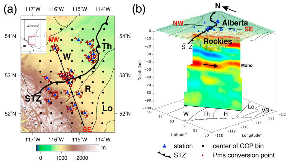
Figure 7. (a) A tectonic map of western Snowbird Tectonic Zone (Ross et al., 1993). The blue triangles mark the seismic stations used in the construction of common conversion point (CCP) gathers. The black circles indicate the centers of the CCP bins, and the red circles denote the P -to- S conversion locations at 40-km depth. The black line shows the location of the receiver function transect. The map area is shown by the enclosed region in the inset. (b) A 3-D perspective plot of the receiver function transect extracted from the CCP gathers. Red and blue colors represent the positive and negative amplitudes, respectively. The Moho is delineated by a positive ( P ms ) phase at ~40-km depth, and its dipping direction beneath the Snowbird Tectonic Zone is indicated by the arrow.
