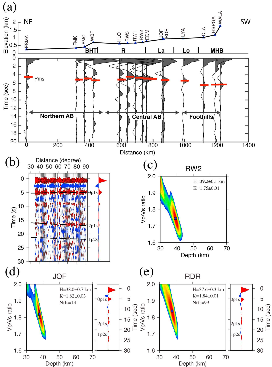
Figure 4. (a) A profile of stacked receiver functions (RFs) showing Moho variations from northern Alberta to the foothills of the Rocky Mountains (see Figure 2a for profile location). Station located within 50 km distance of the profile, which approximately equals the lateral resolution of the RF, are projected on the profile. The elevation and name of each station are indicated above the RF. The red line marks the Pms phase. (b) RFs from station RW2. The dashed black lines mark the predicted arrival times of converted phases from H-k analysis. The stacked trace is shown on the right panel. (c) The H-k diagram of RFs from station RW2. (d and e) The H-k diagrams for two stations (JOF and RDR) that are 8.5 km apart. The stacked RFs are shown on the right-hand side.
