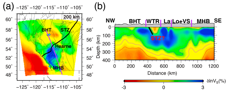
Figure 8. (a) Shear velocity perturbations at 200-km depth from finite-frequency travel time tomography (Gu et al., 2016). The blue diamonds show the location of xenoliths (Buhlmann et al., 2000; Canil et al., 2003; Aulbach et al., 2004). (b) A cross-section of shear velocity profile. Its location is indicated by the purple line in (a), and the potential subsurface extension of the Snowbird Tectonic Zone is indicated by the thick black line. The domain boundaries are marked by the purple lines near the surface. WTR represents the region across the Snowbird Tectonic Zone that includes the Wabamum, Throsby, and Rimbey domains. See Figure 1 caption for other abbreviated domain names.
