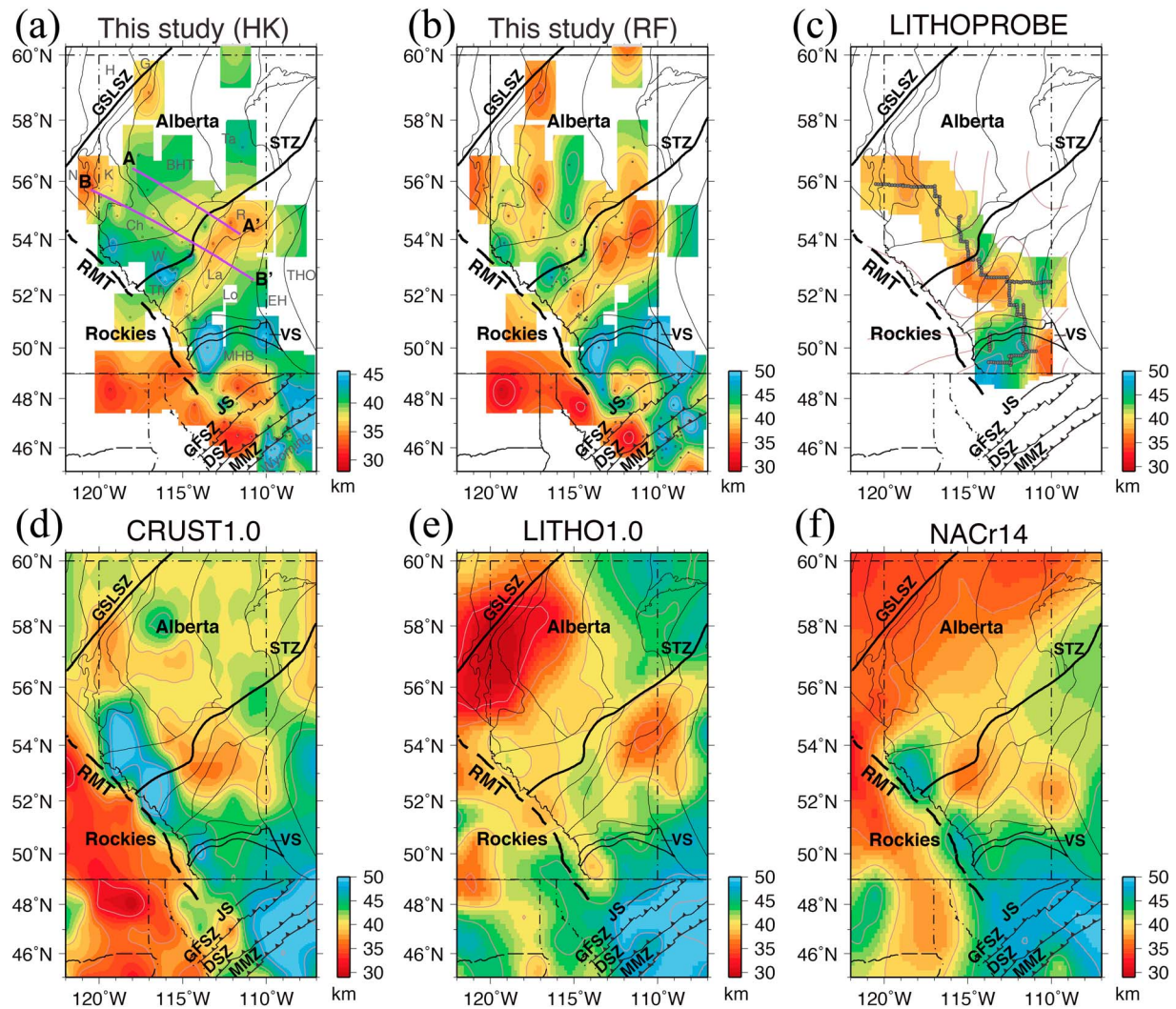
Figure 5. Maps of Moho depth from (a) H-k stacking (this study), (b) time-to-depth conversion (this study), (c) an interpolated map of Bouzidi et al. (2002) based on LITHOPROBE reflection/refraction surveys, (d) CRUST1.0 (Laske et al., 2013), (e) LITHO1.0 (Pasyanos et al., 2014), and (f) NACr14 (Tesauro et al., 2014) models. The locations of two linear transects across the STZ are indicated by the purple lines. The small gray circles indicate the locations of stations. Station elevation is subtracted from crustal thickness ( H ) to calculate the Moho depth.
