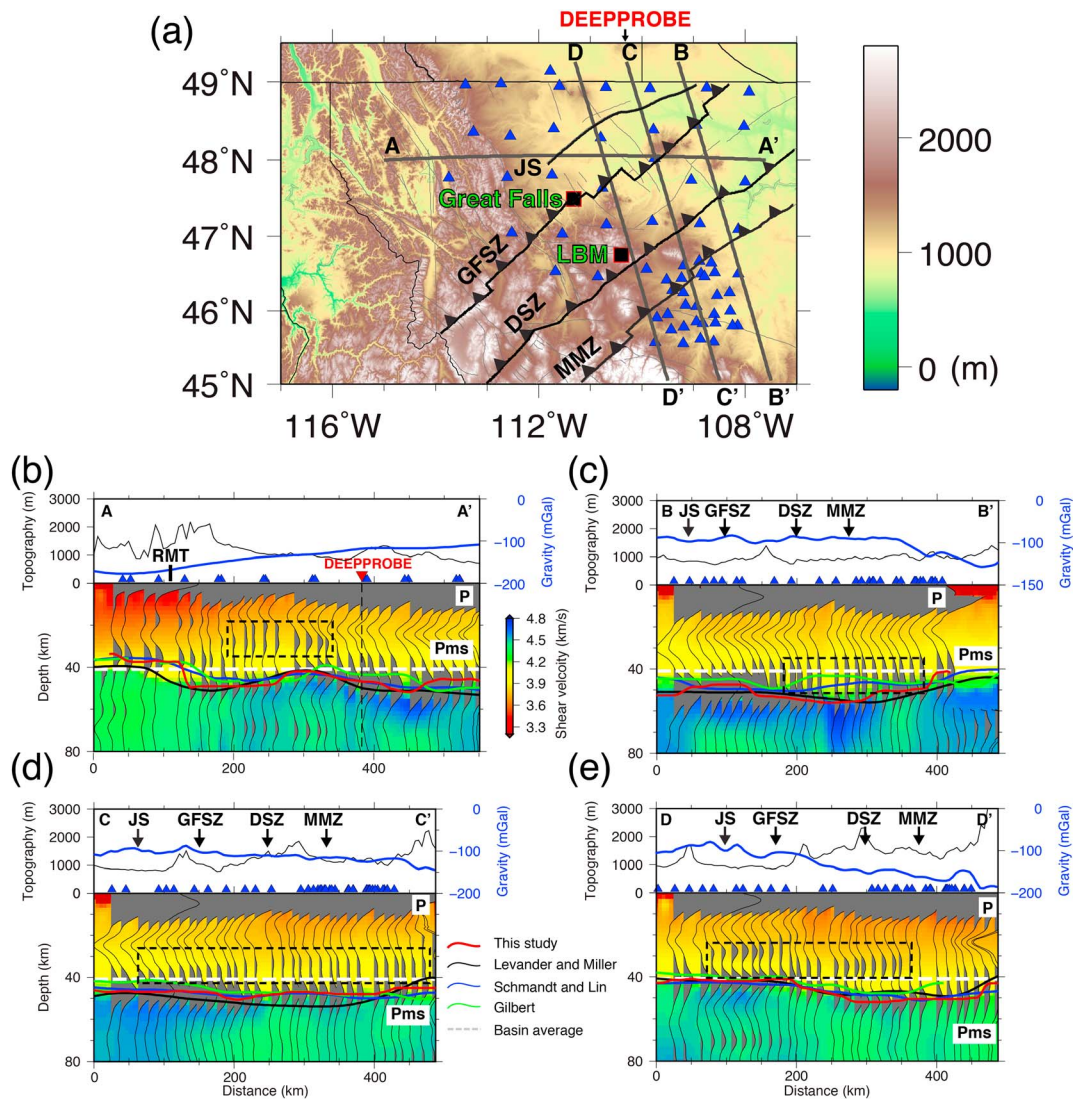
Figure 9. (a) Surface topography near the Great Falls Tectonic Zone in northwestern United States. The blue triangles mark the station locations, and thin black lines indicate four major northeast orientated faults. (b–e; top) Topography (black) and Bouguer gravity (blue) along the profiles shown in (a). The intersections between known faults and seismic profiles are highlighted by the arrows. (bottom) RF transects constructed from the CCP gathers. The background color shows the shear velocities from Shen and Ritzwoller (2016). The solid lines track the Moho depth obtained from this (red) and earlier (Gilbert, 2012; Levander & Miller, 2012; Schmandt & Lin, 2014) studies. The averaged Moho depth in the Alberta basin is shown by the white dashed line. In general, stations with delayed, high-amplitude Moho conversions are underlain by above-average shear velocities. The stacked traces from these stations often show waveform broadening or multiple arrivals (enclosed by the dashed rectangles).
