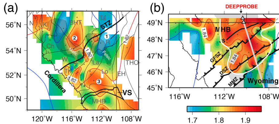
Figure 11. Vp/Vs ratios near the (a) Snowbird Tectonic Zone and (b) Great Falls Tectonic Zone. Labels 1–3 highlight the major anomalies. The DEEPPROBE refraction transect and shot points (Henstock et al., 1998; Gorman et al., 2002; Clowes et al., 2002) are indicated by the white line and grey triangles, respectively. The shaded areas show the reported mafic and felsic magmatic intrusions from earlier geophysical studies (Bouzidi et al., 2002; Chen et al., 2015; Ross, 2002; Ross & Eaton, 1997; Welford & Clowes, 2006). The region of underplating (i.e., lower crustal layer) inferred from elevated Vp/Vs ratios is enclosed by the white line.
