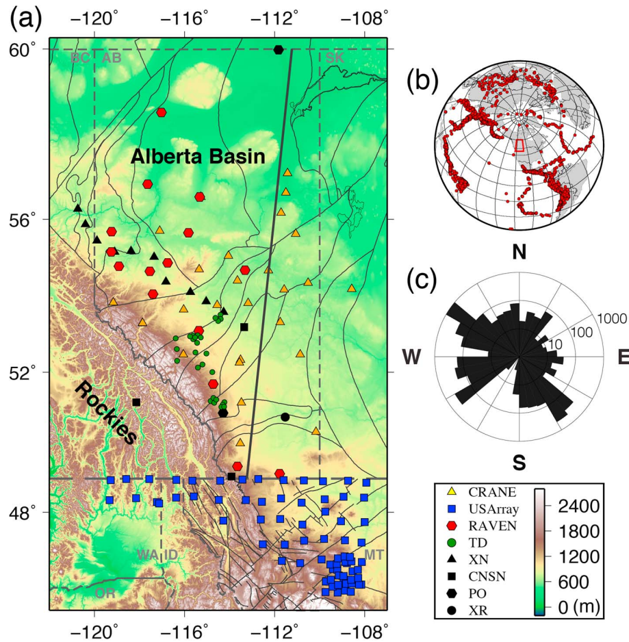
Figure 2. (a) Distribution of regional seismic stations examined in this study. The thin black lines indicate the tectonic boundaries within the Western Canada Sedimentary Basin and fault networks in northern Montana. The thick black line marks the location of a receiver function profile shown in Figure 4a. (b) Earthquakes (red circles) analyzed in this study. The study region is indicated by the red-colored polygon at the center of map. (c) A rose diagram (in logarithmic scale) showing the azimuth distribution of the earthquakes.
